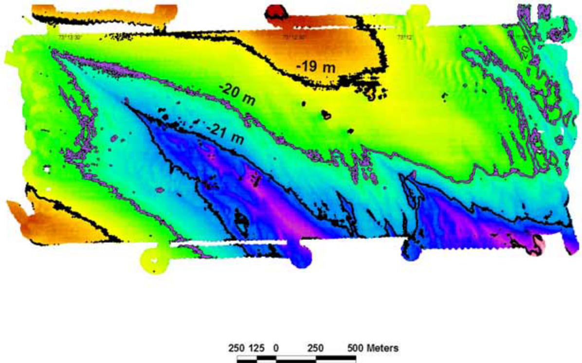
Figure 2. Fire Island Reef January 2005. Contours in meters. Depth decreases towards the top of the figure.
