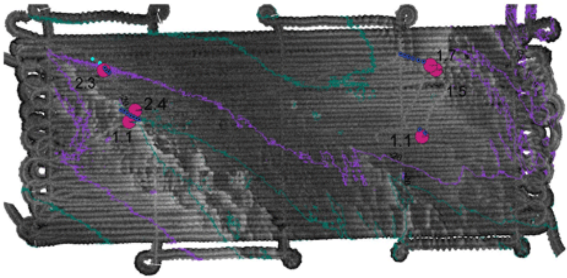
Figure 8b. August 2001 Backscatter map and contours
