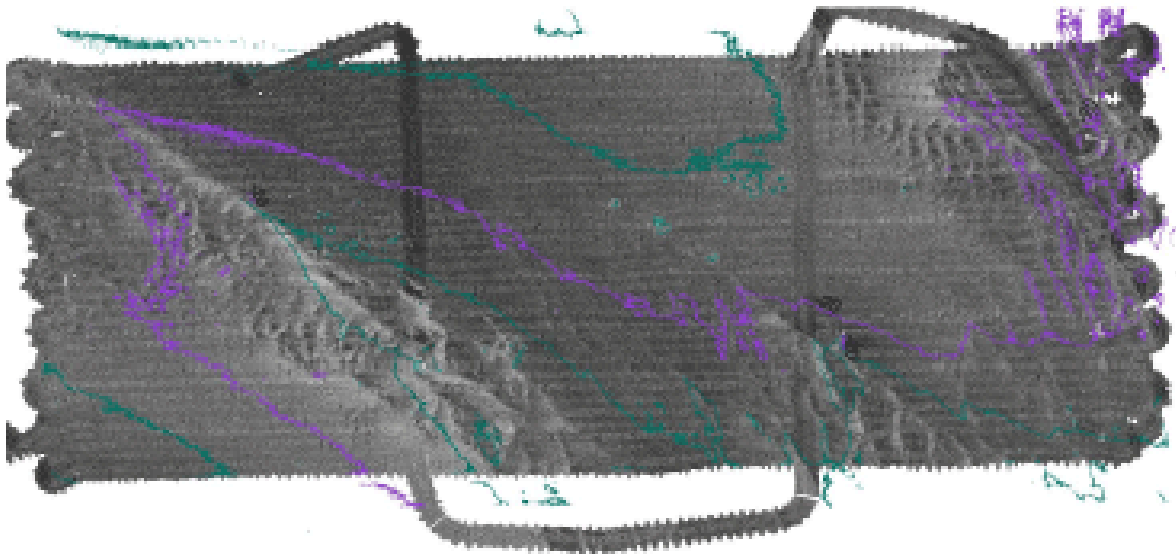
Figure 8b. August 2001 Backscatter map and contours
