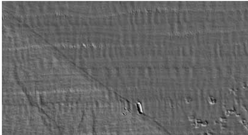
Figure 6b. Shaded relief map showing a planar view of the smooth texture visible in polychaete area during August 2001
