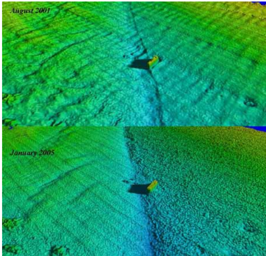
Figure 7. Angled view of the texture change visible in the bathymetry of the polychaete area between August 2001 and January 2005.
