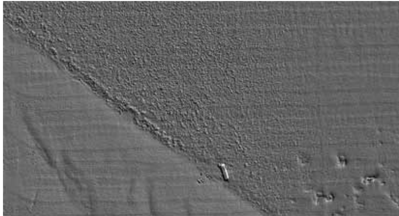
Figure 6a. Shaded relief map showing a planar view of the lumpy texture visible in polychaete area during January 2005
