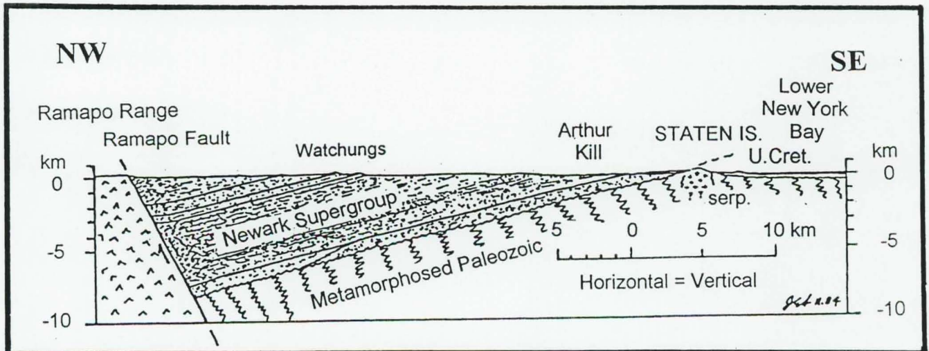
Figure 2 - Profile section from Staten Island to the Ramapo fault showing tilted- and eroded remnants of Newark basin-filling strata. Serp., Staten Is. serpentinite; subsurface relationships not known (J. E. Sanders.)
