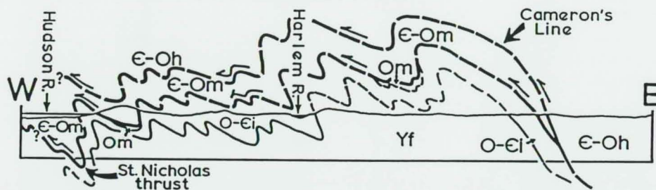
Figure 2 - Geologic map of Manhattan and the Bronx showing a new interpretation of the structure of the Manhattan Schist (adapted from Merguerian and Baskerville, 1987). Notation very similar to figure 1 and inset which shows a new interpretation of the stratigraphy of the region. The east-west geologic section shows the distribution of various tectonostratigraphic units in New York City and geometry of the deformed ductile faults (Cameron's Line and the St. Nicholas thrust).
