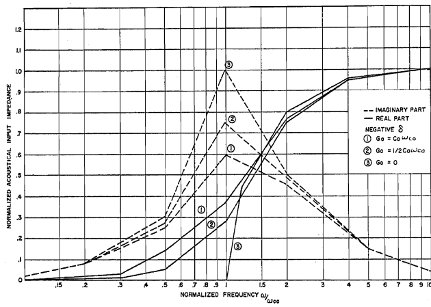
Fig. 4. Normalized acoustical input impedance vs. frequency for negative \delta .
