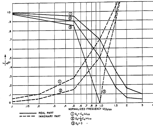
Fig. 2. Real and imaginary parts of \Gamma/(\delta/2) vs. \omega/\omega_{co} .
