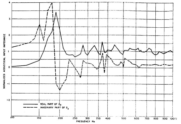
Fig. 5. Measured normalized acoustical input impedance for K-coupler shown in Fig. 1.
