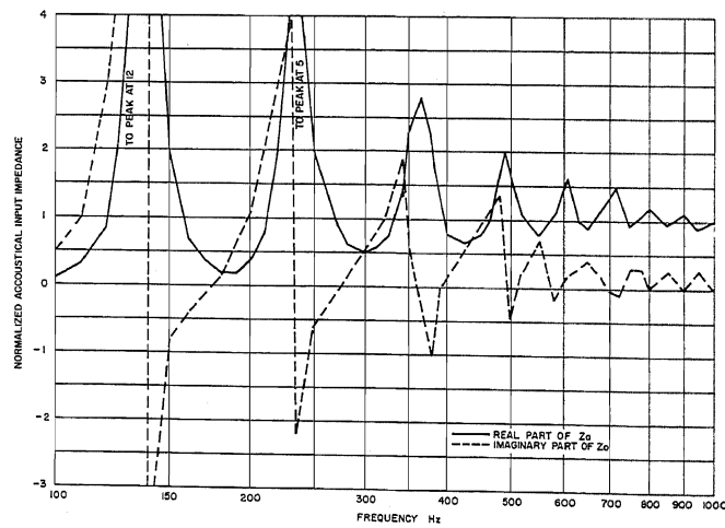
Fig. 6. Calculated normalized input impedance for an exponential horn of comparable dimensions.
