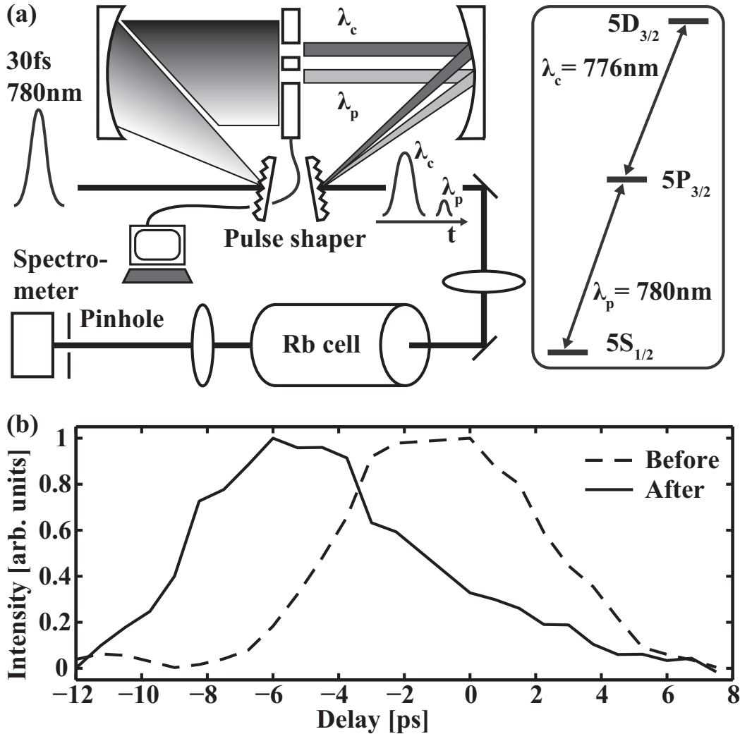
Figure 7.1: (a) shows the experimental setup. A 30 fs pulse was used by the pulse shaper to create two narrow-bandwidth pulses resonant on the coupling and probe transitions at 776 nm and 780 nm, respectively, that were delayed with respect to one another by up to \pm 20 ps. They were focused into the Rb cell and measured with a spectrometer. (b) shows the temporal cross-correlation of probe and coupling pulses before (dashed) and after (solid) the cell.
