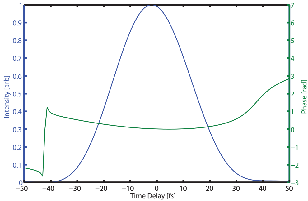
Figure 2.2: Pulse from our laser amplifier. The pulse was characterized using SHG FROG [41].
