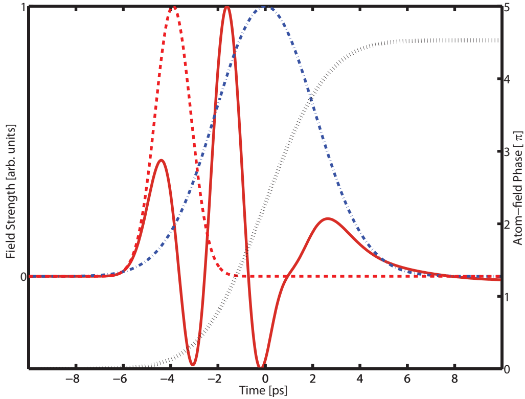
Figure 7.4: Calculated probe and coupling fields and the atom-field phase given by Eq. (7.3). The red-dashed and red-solid lines show the calculated probe pulse envelope before and after the cell, respectively. Both curves are normalized to their peak values. The black-dotted line is the atom-field phase, \alpha(t) . The blue-dashed-dot line is the normalized coupling pulse.
