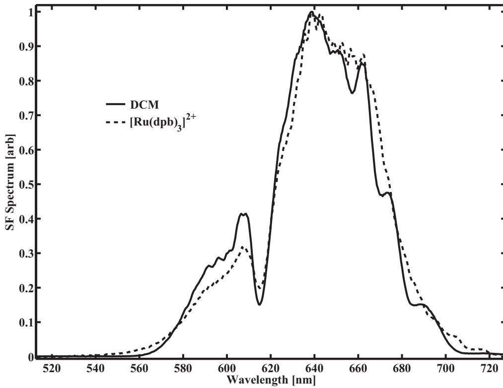
Figure 8.4: Normalized superfluorescence spectra from the two-photon absorbing dyes for an unshaped pulse. The solid curve represents emission from DCM and the dashed curve represents emission from [\text{Ru}(\text{dpb})_3]^{2+} .
