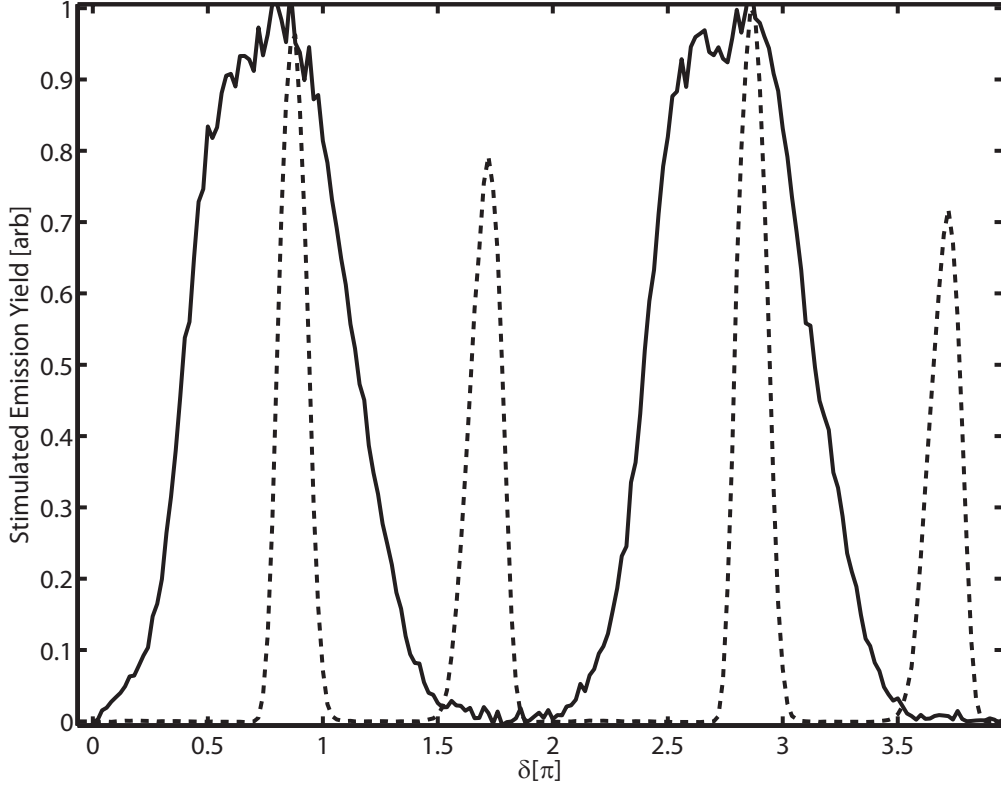
Figure 8.7: Normalized lineouts of Fig. 8.6. The solid curve represents superfluorescence for Rb and the dashed curve for Na. The yields are normalized and represent different energies.
