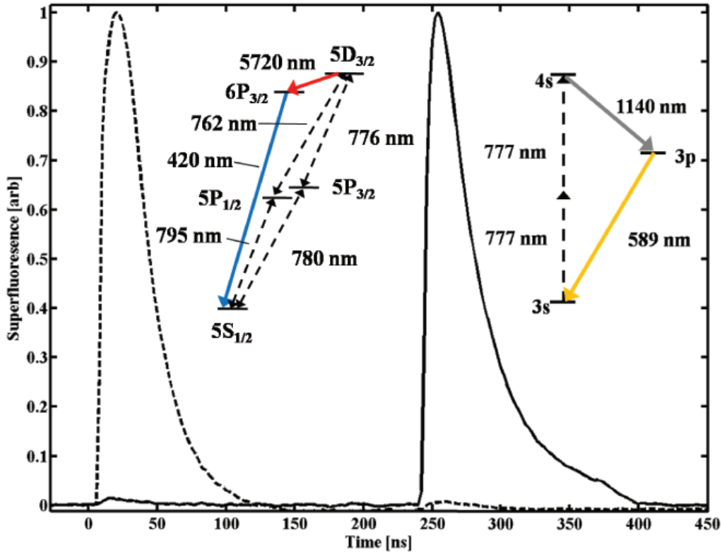
Figure 8.2: Normalized control results for selectivity between Rb and Na stimulated emission. The solid curve represents a pulse designed to maximize Na/Rb and the dashed curve represents a pulse designed to maximize Rb/Na. The signal starting at \sim 0 ns represents Rb and that at \sim 250 ns, Na. The insets show the atomic level structure, where the blue line is the lasing we measure in Rb and the orange line is the lasing we measure in Na. The pulse energies were approximately 170 \mu\text{J} for Na and 45 \mu\text{J} for Rb.
