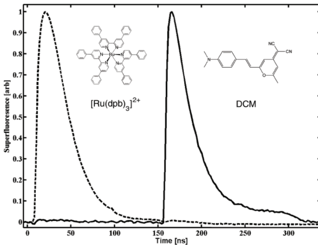
Figure 8.5: Normalized control results for selectivity between DCM and [\text{Ru}(\text{dpb})_3]^{2+} . The solid curve represents a pulse designed to maximize \text{DCM}/[\text{Ru}(\text{dpb})_3]^{2+} and the dashed curve represents a pulse designed to maximize [\text{Ru}(\text{dpb})_3]^{2+}/\text{DCM} . The signal starting at \sim 0 ns represents [\text{Ru}(\text{dpb})_3]^{2+} and that at \sim 150 ns, DCM. The insets show the two chemical structures of the molecules.
