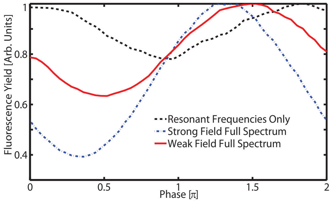
Figure 6.2: 5D population as a function of spectral phase on the 775.94\text{ nm } 5P_{3/2} \rightarrow 5D_{3/2} transition. The dotted black curve corresponds to the case where only the resonant frequencies in the broadband pulse were present and all other frequencies were blocked. The solid red curve corresponds to weak field excitation with full spectrum and the blue dot dashed corresponds to strong field excitation with the full spectrum.
