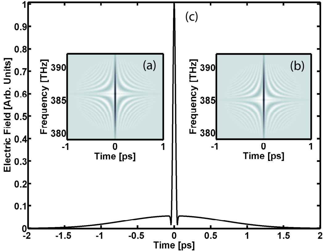
Figure 6.4: Wigner plots of the phase shaped pulses. (a) The Wigner plot of a pulse with the phase window located at 775.94 nm (386.6 THz). (b) The Wigner plot of a pulse with the phase window located at 780.02 nm (384.6 THz). (c) The electric field envelope associated with (a) and (b).
