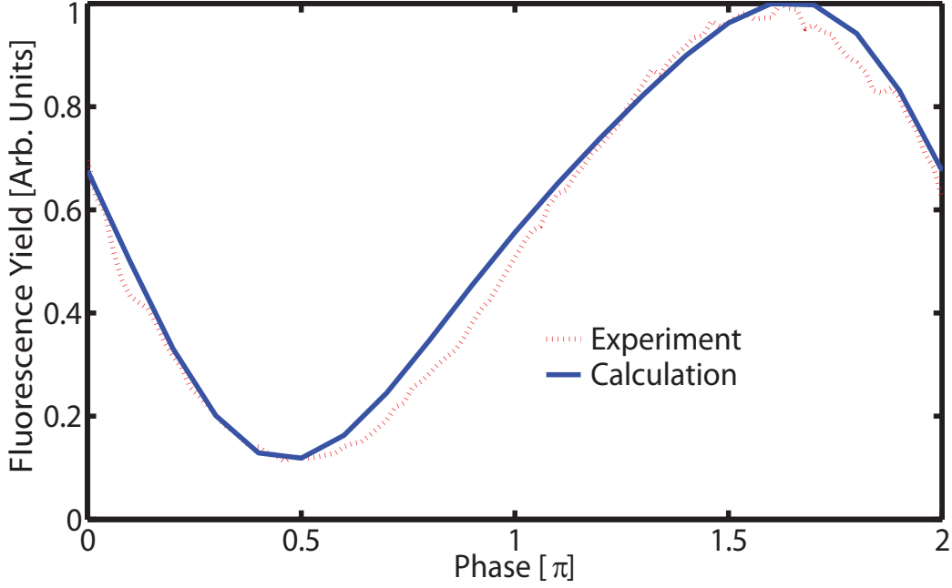
Figure 6.3: Measured and calculated 5D population as a function of phase applied to 794.76 nm while blocking 780.02 nm in the case of the full laser spectrum.
