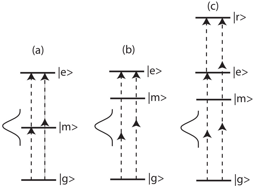
Figure 1.1: Two and three-photon absorption. The laser bandwidth is illustrated at the left showing that multiple frequencies can add in a multiphoton transition. (a) Two-photon absorption between a ground state |g\rangle and excited state |e\rangle through a resonant intermediate state |m\rangle . (b) The same as (a), where the intermediate state |m\rangle is far from resonance. (c) (2+1) Three-photon absorption where there is a two-photon absorption through an off-resonant intermediate state |m\rangle followed by a single photon absorption to a resonant state |r\rangle .
