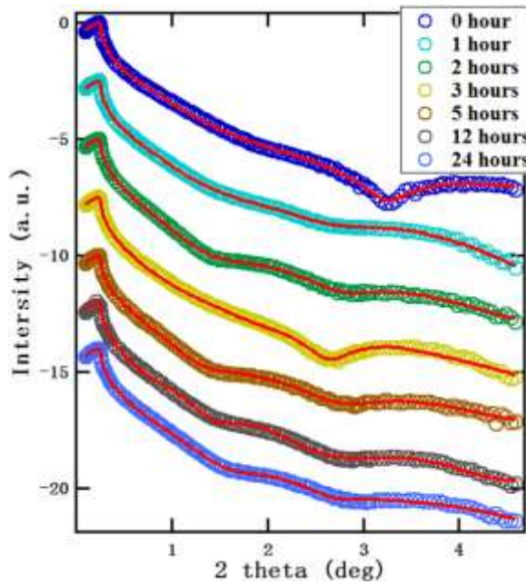
Figure 3-4 X-ray reflectivity data for the adsorbed layer is shown as symbols with fittings as lines for the films that are annealed at 85°C for different time.
