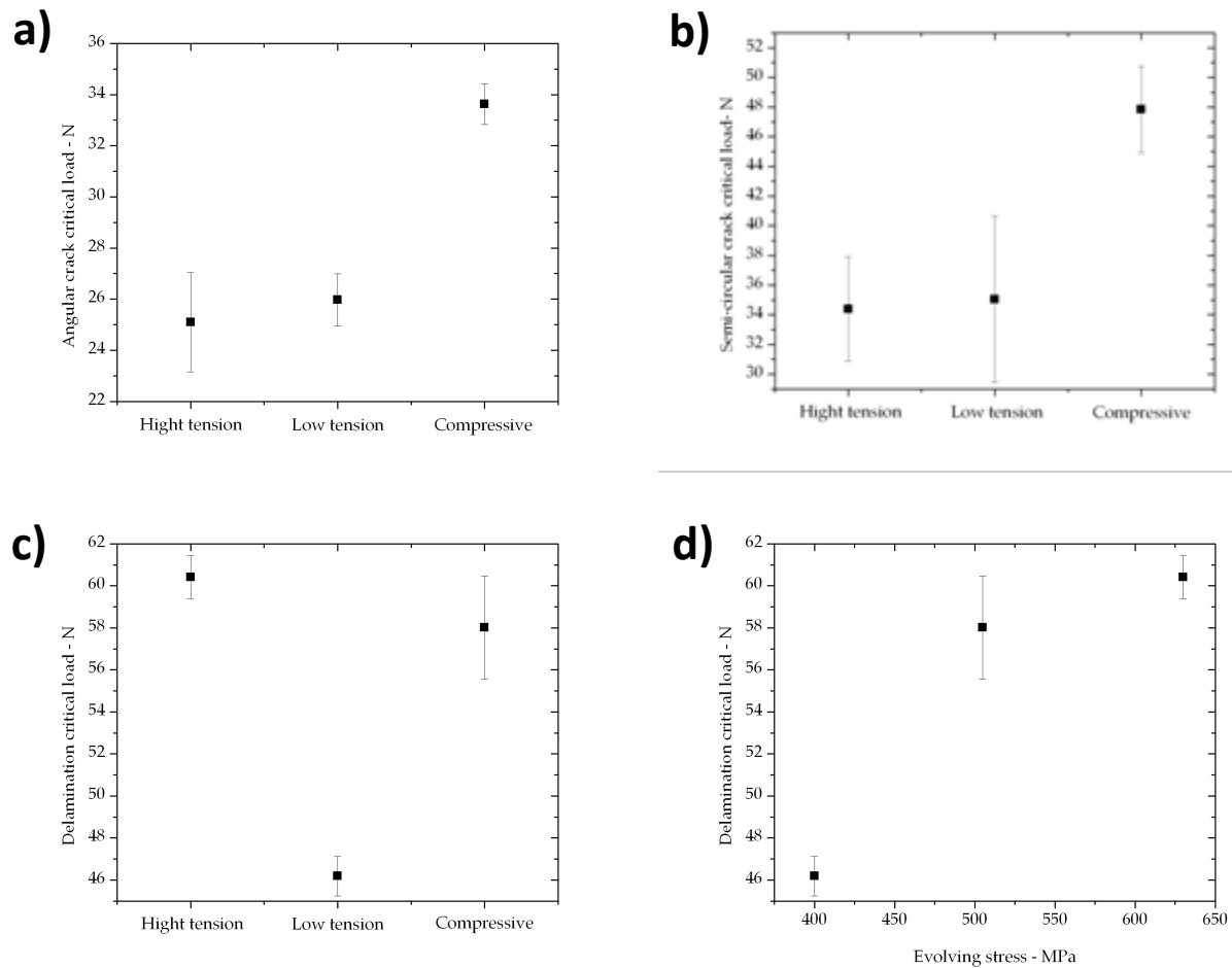
Figure 6.16: Angular critical load (a), semi circular critical load (b), delamination critical load (c) versus different residual stresses and delamination critical load versus different evolving stresses (d)
