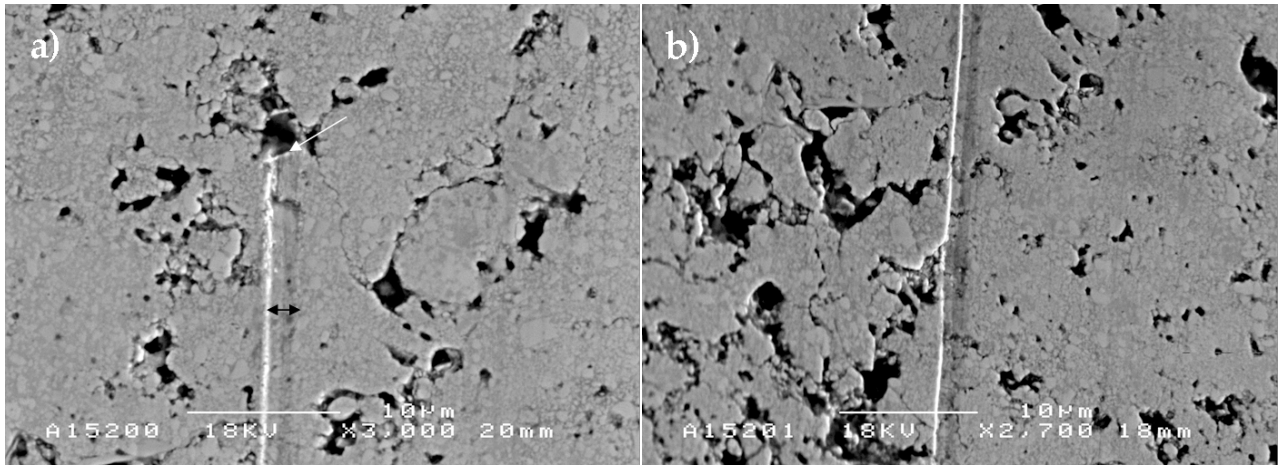
Figure 5.16: (a) single scratch caused by \text{SiO}_2 abrasive particle started from surface open porosities, (b) continuation of same scratch and (c) schematic of scratches formed on the surface of material and started from surface open porosities
