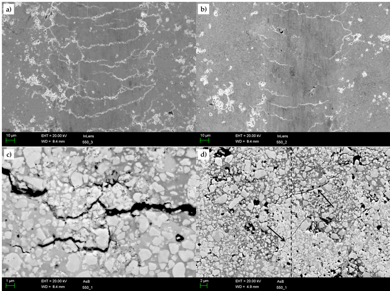
Figure 6.12: SEM studies of scratch groove for coatings deposited with cold (a) and hot (b) and (c) details of semi-circular crack and (d) angular cracks (scratch direction bottom to top)
