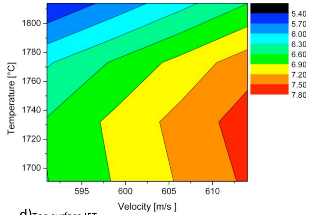
Figure 4.20: Correlation of in-flight particles temperature and velocity to properties and performance; (a) ICP elastic modulus (GPa), (b) hardness, (c) cross section indentation fracture toughness ( \text{MPa}\cdot\text{m}^{0.5} ), (d) top surface indentation fracture toughness ( \text{MPa}\cdot\text{m}^{0.5} ) and (e) rubber wheel abrasion in ( \text{mg}/30\text{min} )
