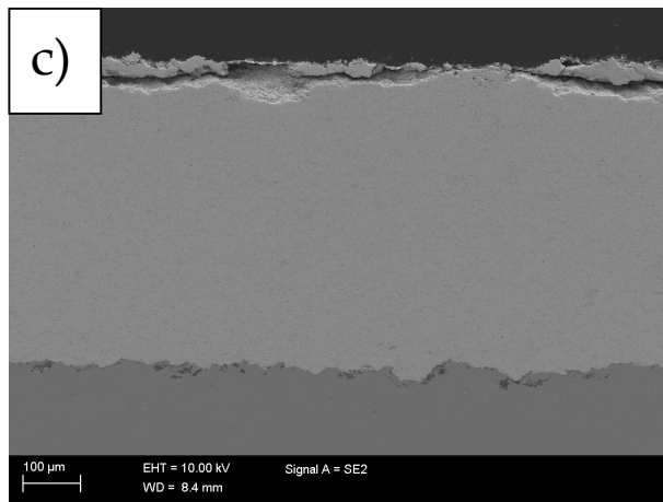
Figure 5.9: SEM microstructural images of (a)conventional, (b)sub-micron and (c)nano coatings deposited by CJS
