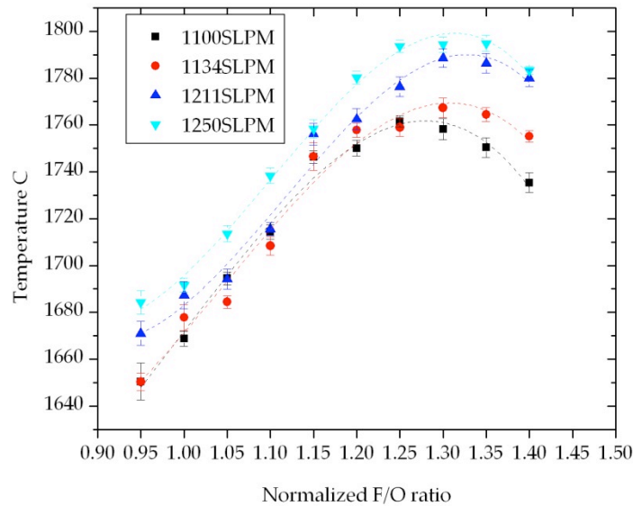
Figure 4.5: Temperature versus normalized F/O ratio under controlled total volume flow condition
