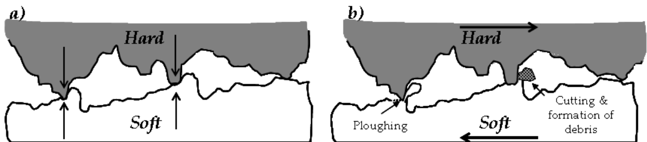
Figure 2.4: Schematic of abrasive wear mechanism of soft surface by hard surfaces in contact: a) Contact of hard surface asperities with soft surface, b) Plowing and cutting of soft material by asperities of harder surface.
