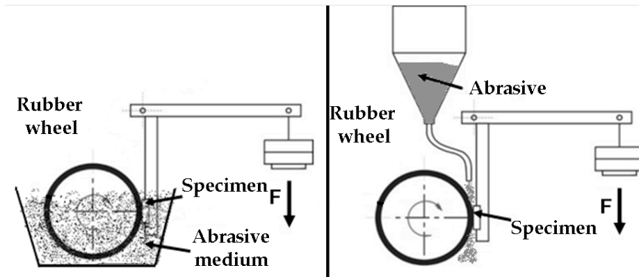
Figure 5.2: Schematic of settings used in this study for slurry abrasion test (left) and dry abrasion test (right)
