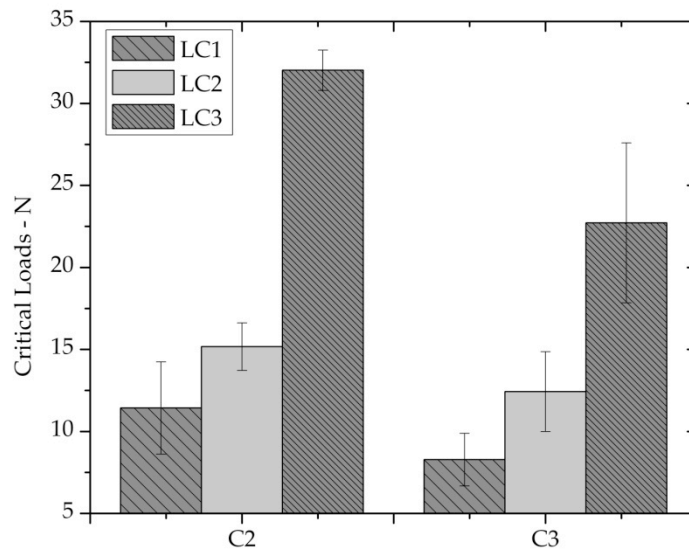
Figure 6.11: Critical loads for coatings deposited with low and high temperature
