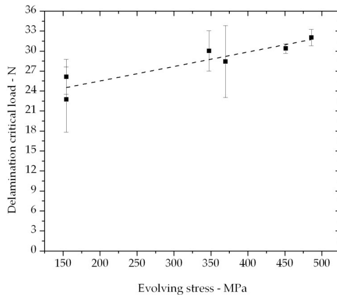
Figure 6.17: Correlation of delamination load and evolving stress for WC-CoCr coatings
