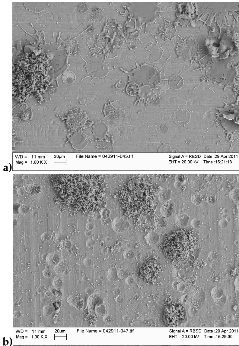
Figure 1.4: CrC-NiCr splats sprayed by APS (high heat input) that shows full decomposition, and HVOF (low heat input) that shows retaining the CrC. In (b) low melting of particles leave the particles in their solid state and cause crater trace on the substrate surface. (Courtesy of Dr. Yikai Chen)
