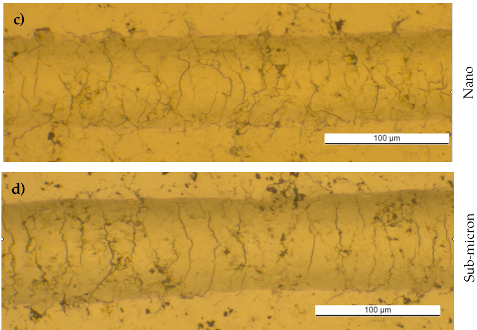
Figure 6.14: Middle of scratch on (c) nano coating and (d) sub-micron coating
