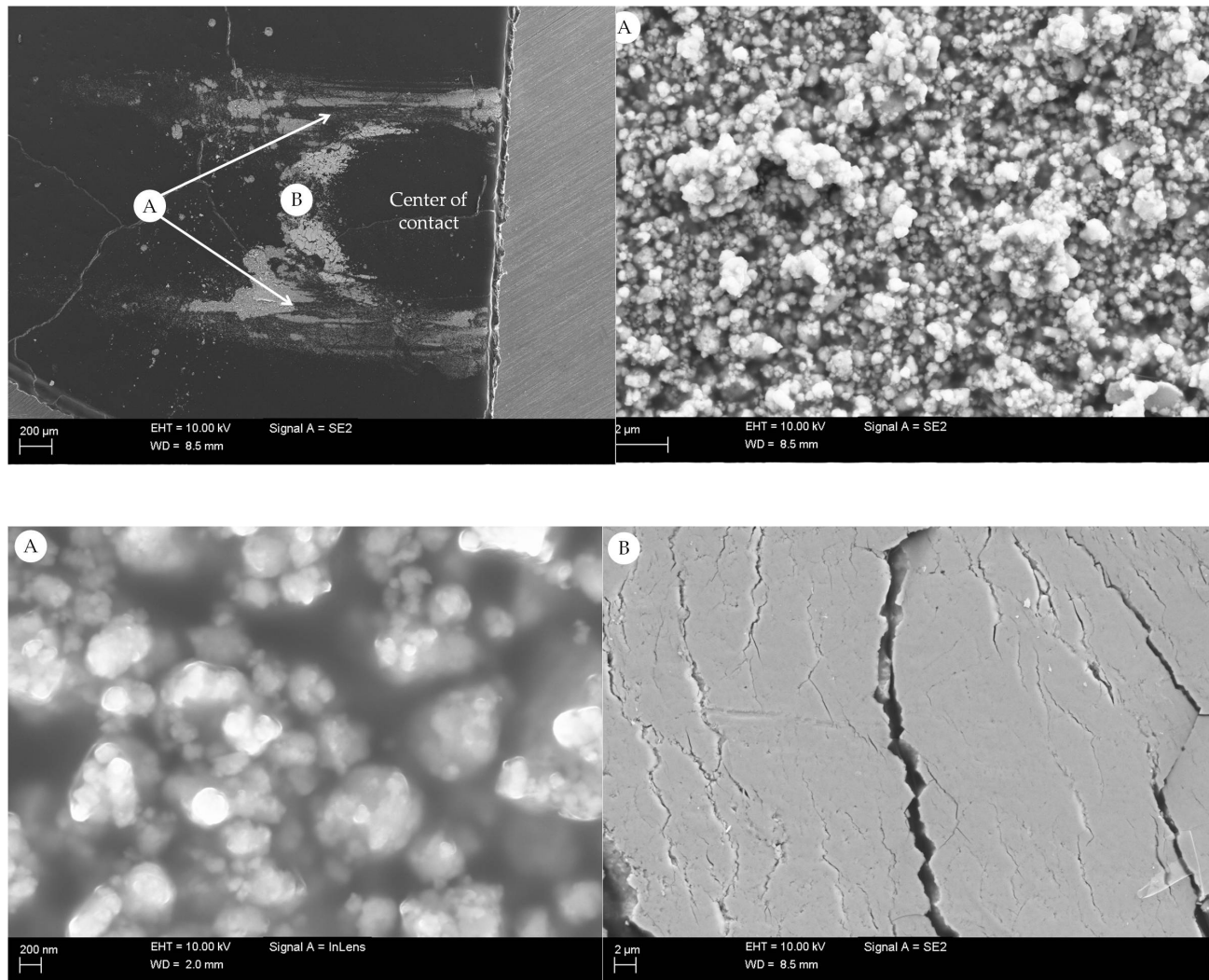
Figure 5.19: Debris collected from two different regions of contact area on carbon tape
