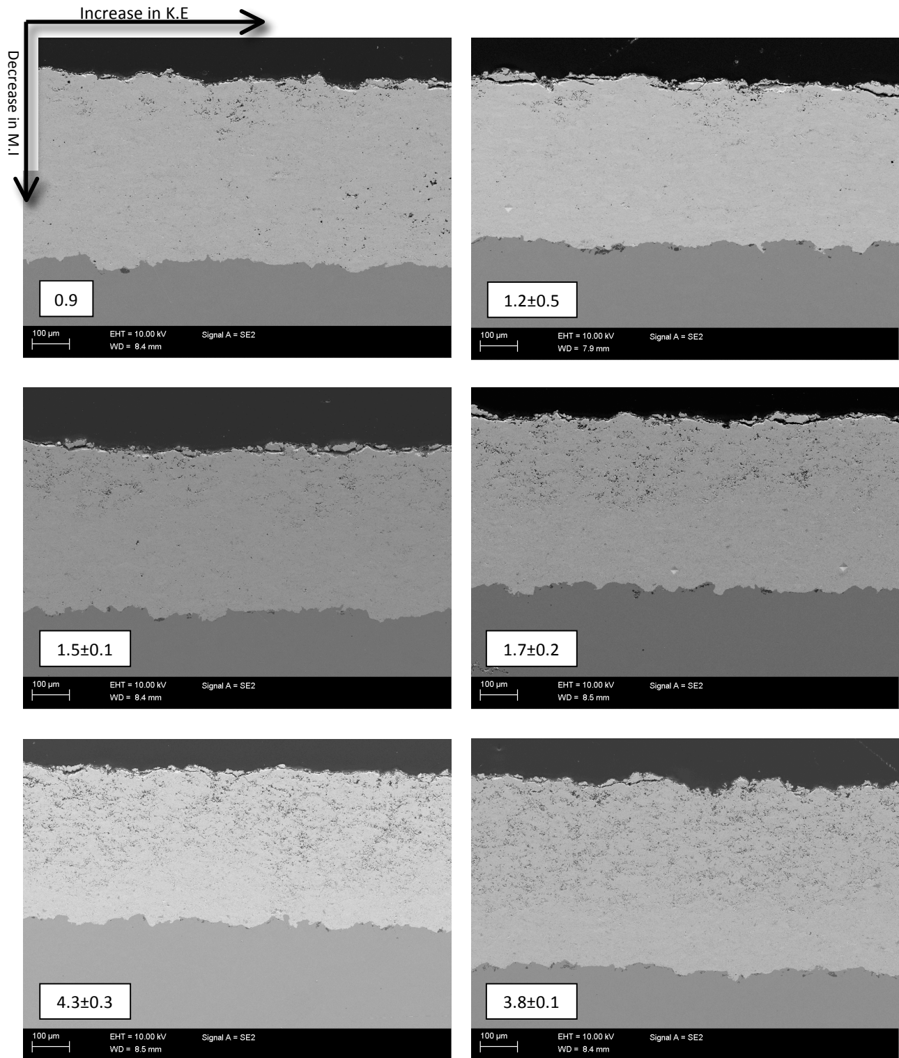
Figure 4.17: Low magnification microstructural SEM images with different M.I. and K.E. values
