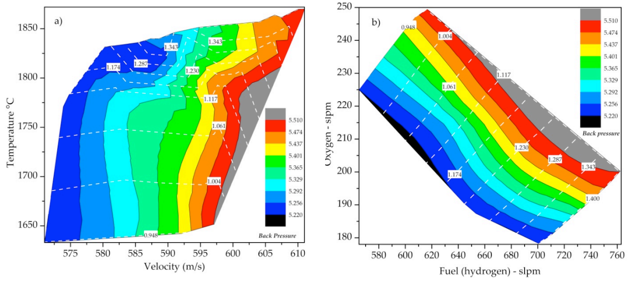
Figure 4.11: Guideline for estimation of a) required back pressure (bar) and \gamma^* to obtain particular T&V and b) a guideline for estimation of required fuel and oxygen value to obtain particular back pressure (bar) and \gamma^* . (b) to (a) is process map route and (a) to (b) is process design route.
