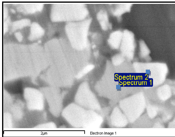
Figure 4.16: EDS study of WC-CoCr coating and corresponding table
