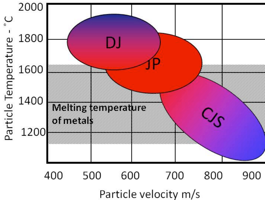
Figure 1.3: Particle temperature and velocity of carbide based coatings applied by different commercially available HVOF systems
