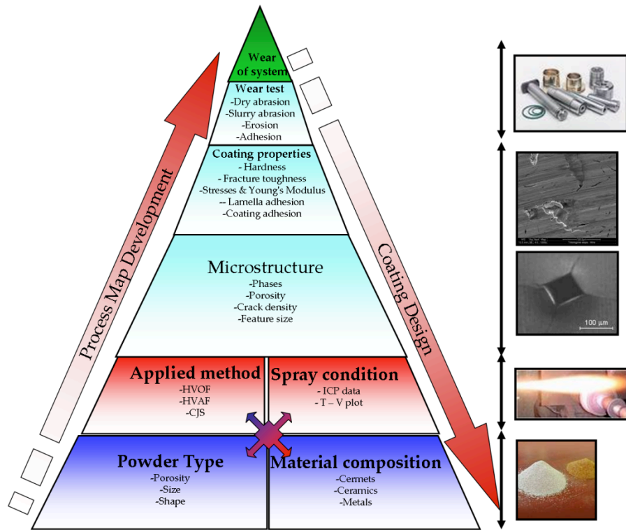
Figure 4.1: Process map, bottom to top, and coating design route, top to bottom for wear performance of a coating/substrate system.
