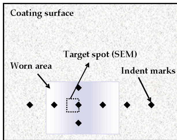
Figure 5.12: Schematic of relocating process and sample preparation
