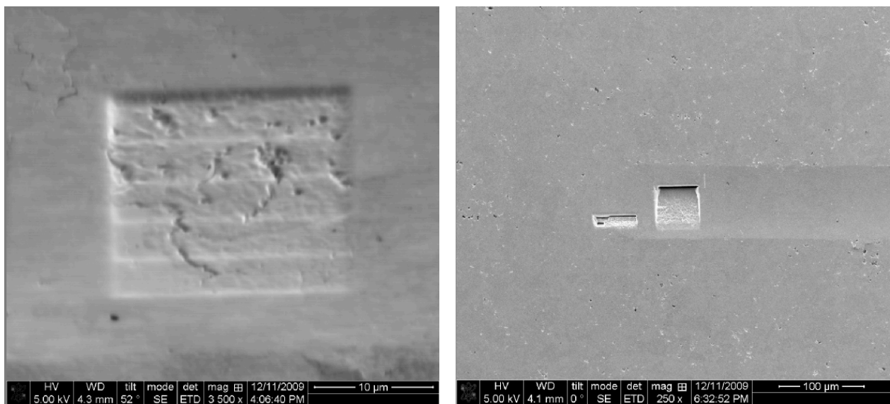
Figure 6.18: Top surface of coating after few minutes of milling (left) and top surface of coating after completed milling (end of scratch groove)
