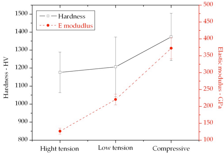
Figure 6.15: Indentation hardness and elastic modulus values for coatings with different residual stress levels
