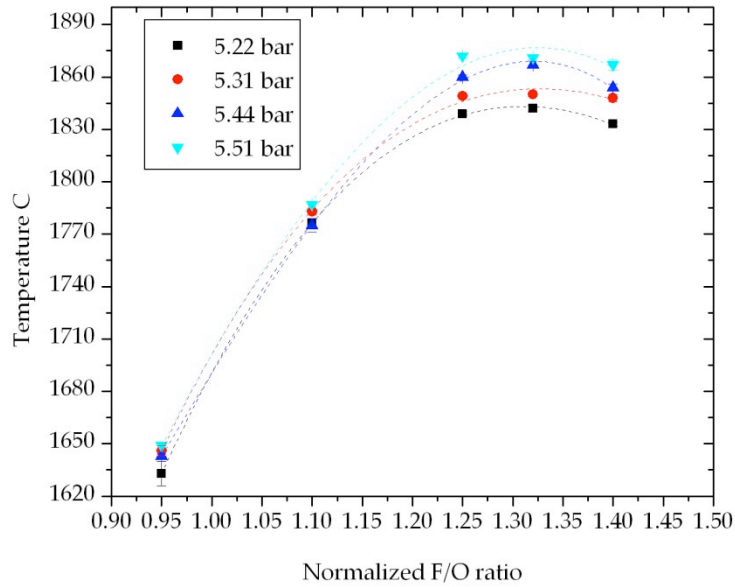
Figure 4.8: Temperature versus normalized F/O ratio under controlled back pressure condition. To address the effect of hydrogen and oxygen separately on measured backpressure as well as on in-flight particles temperature and velocity, it was attempted to control the \gamma^* ratio in two different manners. In one set it was attempted to keep the oxygen constant and change the hydrogen (hydrogen controlled). In second set it was attempted to keep the hydrogen constant and change the oxygen (oxygen controlled). In both cases targeted fuel/oxygen ratios were achieved except for \gamma^*=1.4 in hydrogen controlled and \gamma^*=0.95 for oxygen controlled conditions. The reason not to be able to cover whole range was the limits of torch and employed gas feeding systems. Figure 4.9a shows the effect of hydrogen and oxygen flow (total volume flow) on backpressure. It is shown that changing in oxygen flow has larger impact on backpressure than hydrogen (the slope of oxygen controlled curve is 0.008 and hydrogen controlled curve is 0.002). Figure 4.9b depicts that small changes in back pressure caused by hydrogen provides bigger changes in velocity values. Figure 4.9c examines the validity of same function proposed previously (back pressure multiplied by total volume flow).
