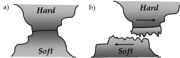
Figure 2.3: Schematic of adhesive wear mechanism: a) Contact of asperities and possible cold welding. b) Fracture of weaker material due to relative movement of surfaces in contact.
