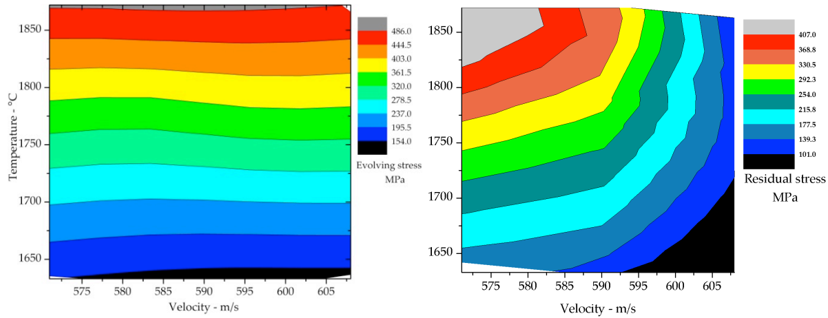
Figure 4.19: Dependency of (left) evolving stress and (right) residual stress on in-flight particles temperature and velocity
