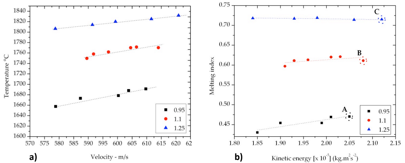
Figure 4.12: a) Measured in-flight particles temperature and velocity at three different \gamma^* levels and b) same points converted to MI-KE space
