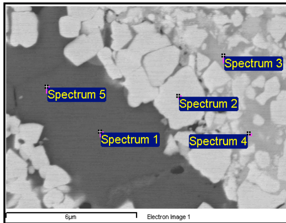
Figure 4.15: EDS study of WC-CoCr coating and corresponding table
