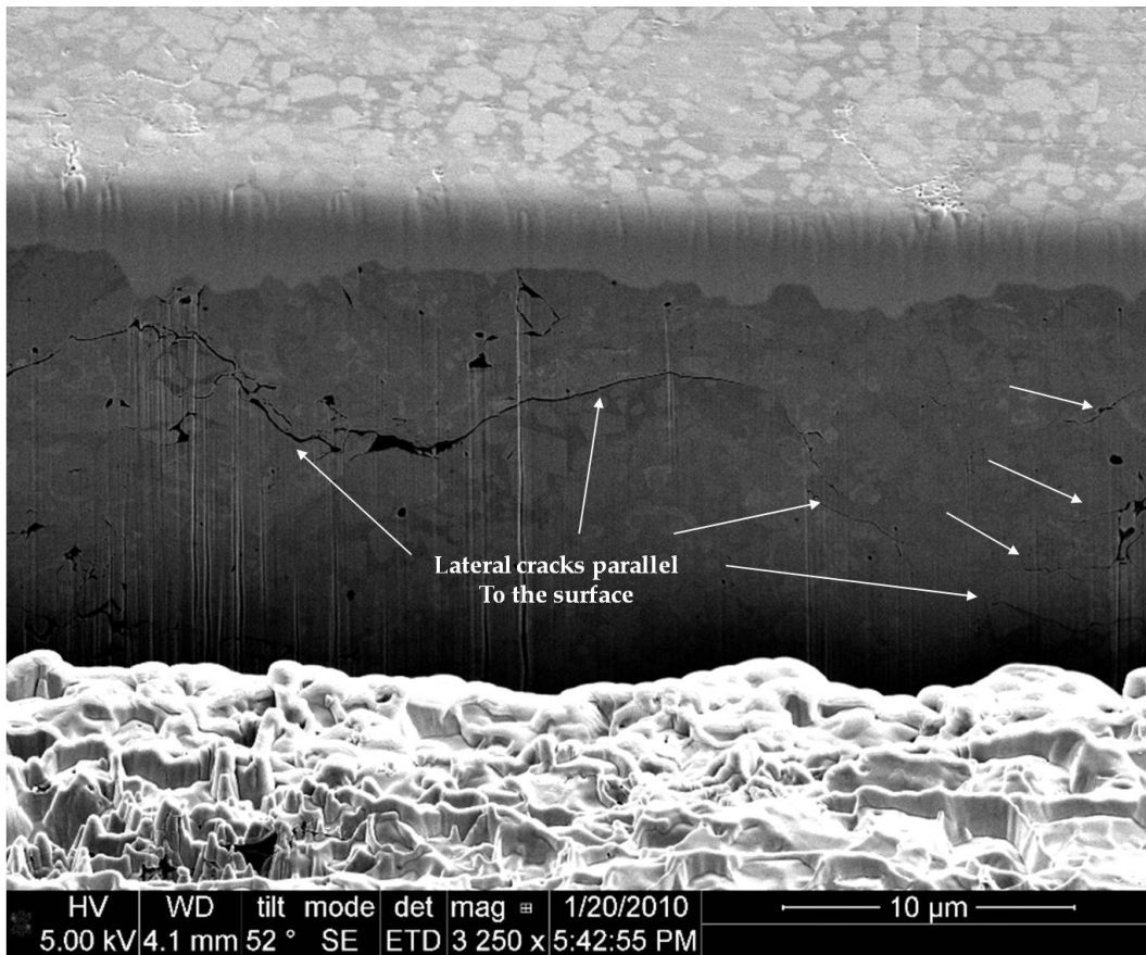
Figure 6.21: Sub-surface cross section of scratch groove on coating under tensile stress
