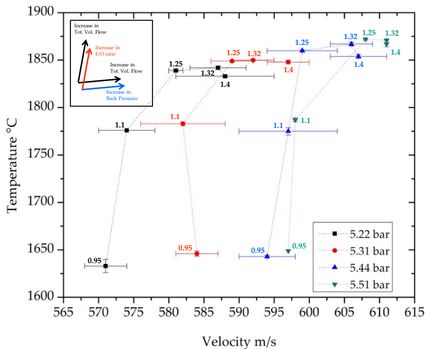
Figure 4.6: In-flight particles temperature and velocity with controlled \gamma^* and back pressure. (table 3.3)
