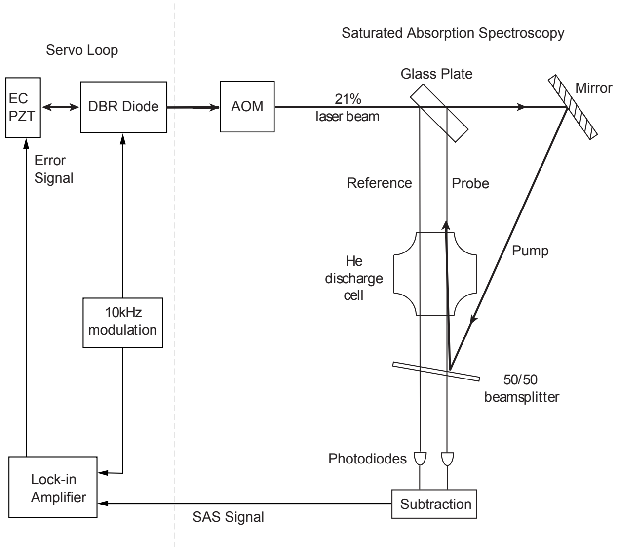
Figure 5.2: Schematic for laser frequency locking to the 2^3S_1 \rightarrow 2^3P_2 transition of \text{He}^* by Saturation Absorption Spectroscopy. The right side of the diagram shows how the SAS signal is derived from the 21% leakage beam of the diode laser. The left side of the figure shows how the SAS signal is used to produce electronic feedback for laser frequency stabilization.
