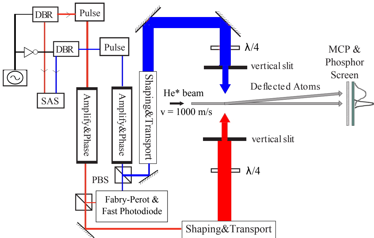
Figure 5.12: Experimental setup for deflection of \text{He}^* with pulsed, chirped light with variable atomic velocity. Diode light is amplitude and phase modulated using EOM's while the frequency of each laser is swept slowly to simulate an atomic velocity. Multiple fiber amplifiers are used to achieve sufficient optical power. The two pulses interact transversely with a \text{He}^* beam sequentially to produce an atomic deflection that is detected using an MCP and phosphor screen.
