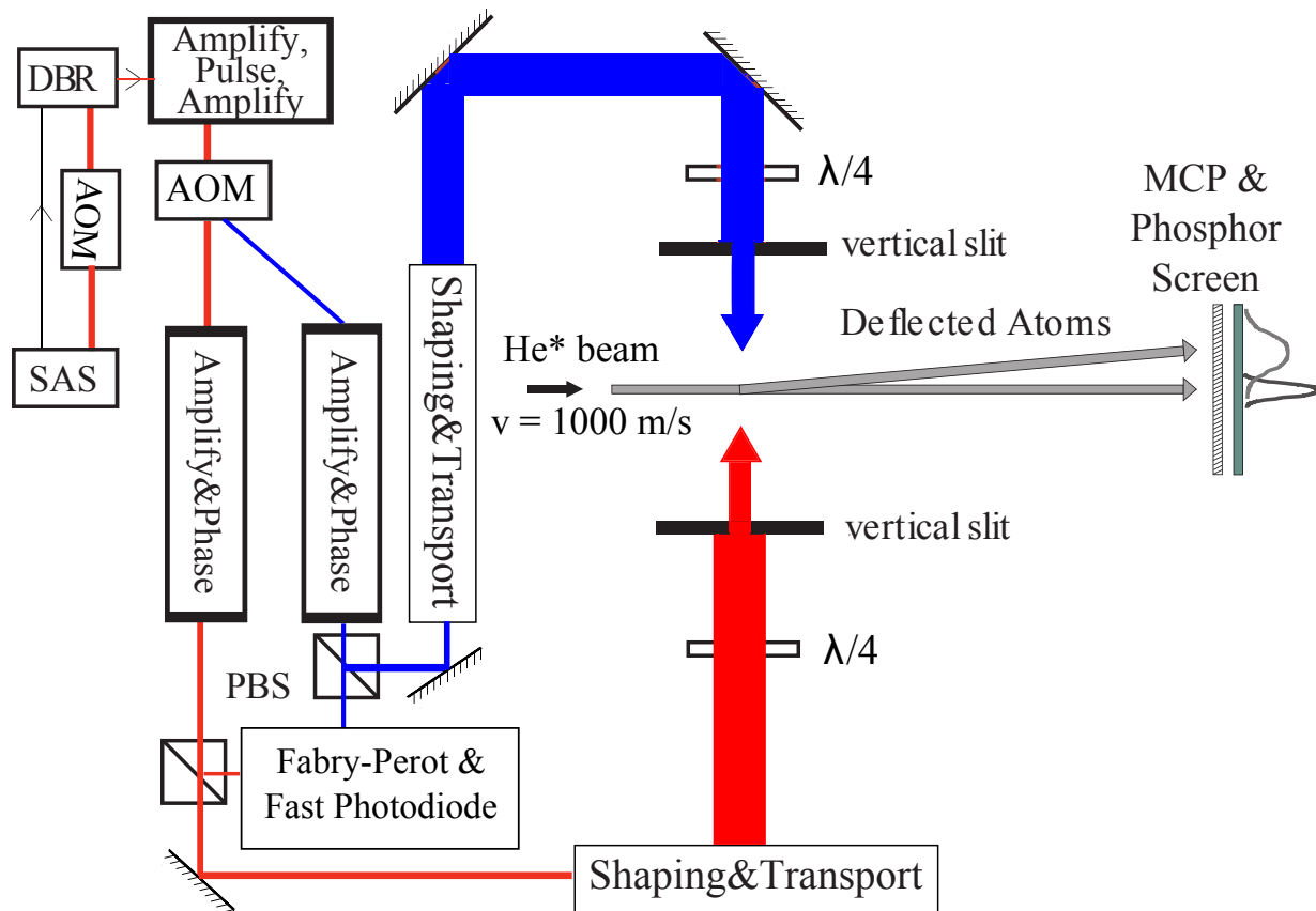
Figure 5.11: Experimental setup for deflection of He* with pulsed, chirped light at a fixed atomic velocity. Diode light is amplitude and phase modulated using EOM's while the absolute frequency is locked at a chosen frequency \delta from atomic resonance. Using both undeflected and deflected beams from an AOM produces two optical beams at frequencies shifted by +\delta and -\delta . More details can be seen in Fig. 5.13. Multiple fiber amplifiers are used to achieve sufficient optical power. The two pulses interact transversely with a He* beam sequentially to produce an atomic deflection that is detected using an MCP and phosphor screen.
