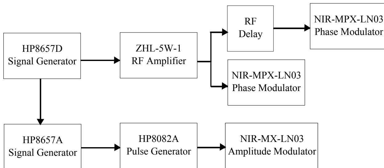
Figure 5.6: RF signal generation for use with EOM's. The RF signal to the NIR-MX-LN03 is supplied by an HP8082A pulse generator triggered by an HP8657A signal generator. The DC voltage is supplied by a Power Design Inc. model 2005 precision power supply. The signal is then amplified by a Mini-Circuits ZHL-5W-1 RF amplifier powered by a Power Design Inc. model 6105 power supply. Afterwards the signal is split into two equal parts with one signal sent directly to a phase modulator and the other is delayed by an RF trombone before it arrives at the other modulator.
