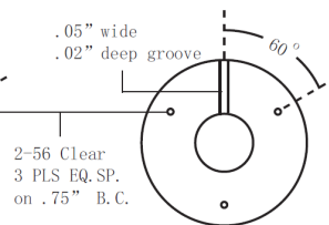
c) right View
