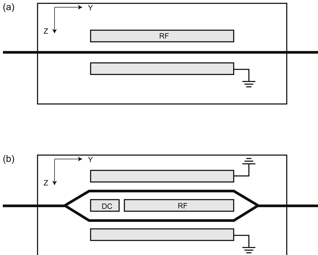
Figure 5.5: Schematic layouts of the NIR-MPX-LN03 phase and NIR-PX-LN03 amplitude modulator ((a) and (b) respectively). The principle axes of the crystal are shown in the corner of the figure.
