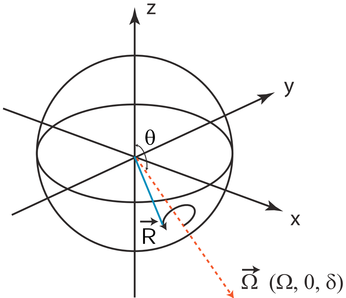
Figure 1.2: Projections of the Bloch and torque Vectors on the Bloch sphere. The solid line represents the Bloch vector \mathbf{R} precessing about the torque vector \vec{\Omega} , represented by the dashed line. Taken from [13]
