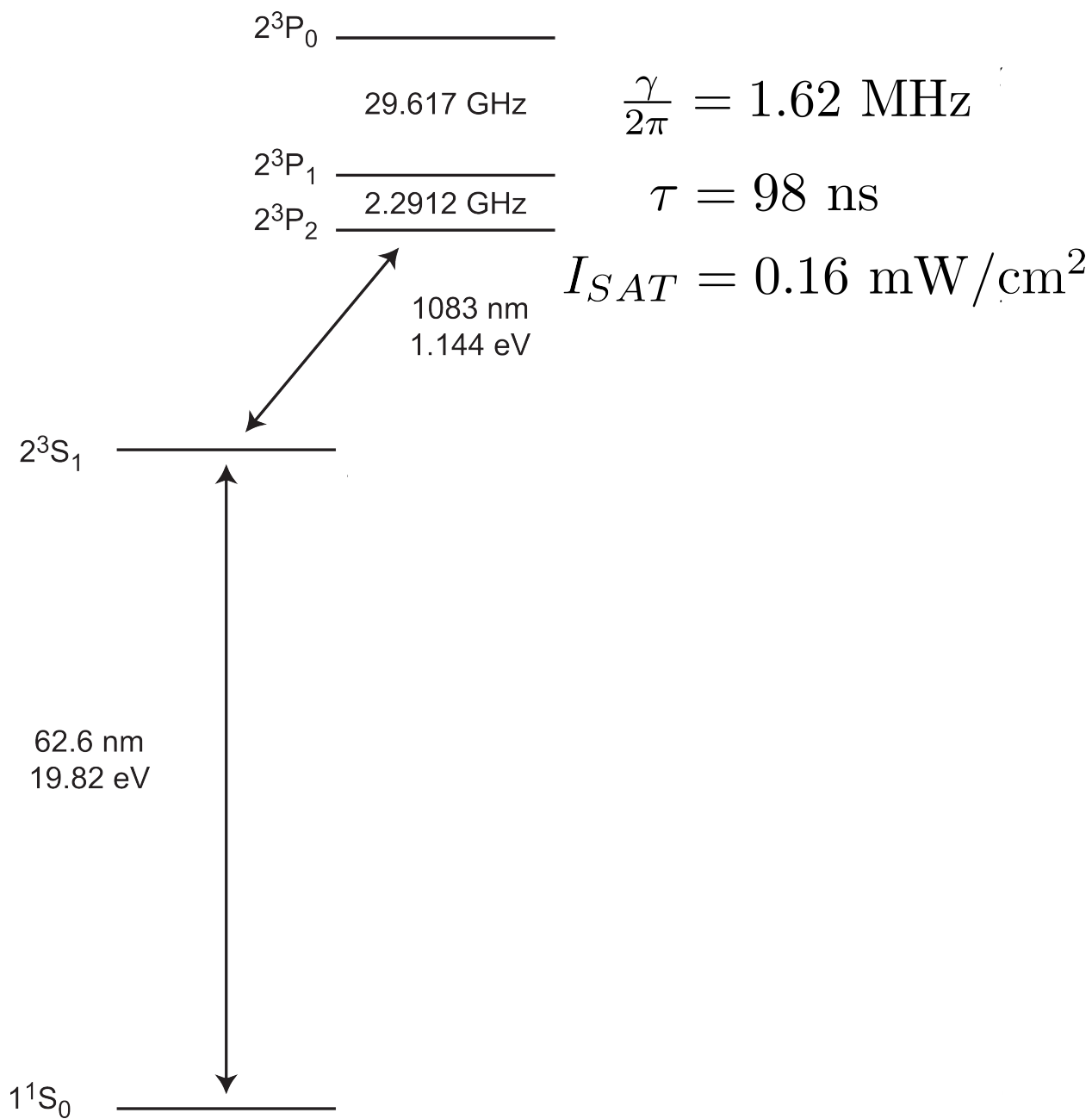
Figure 4.2: Relevant energy levels for the ARP experiments in helium. The lifetime of the metastable state 2^3S_1 is \sim 7900 \text{ s} and serves as the “ground state” for our experiments [58].
