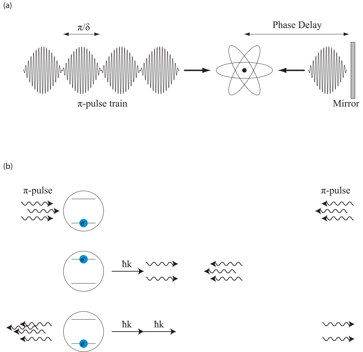
Figure 1.5: The two frequencies in the bichromatic laser beam create a series of \pi -pulses from the beat frequency. Each \pi -pulse excites or de-excites the atom in a time of \pi/\delta leading to a force (\hbar k \delta / \pi) much larger than F_{rad} . Taken from [26].
