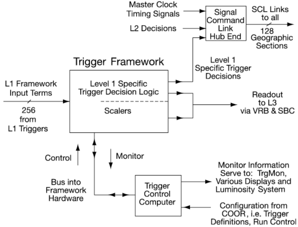
Figure 4.5: A sketch of the D0 trigger frame work. The TFW controls the L1 and L2 trigger decisions and data pipelines. It sends commands to and receive status messages from each component of the L1/L2 trigger systems via a two way serial command line (SCL).
