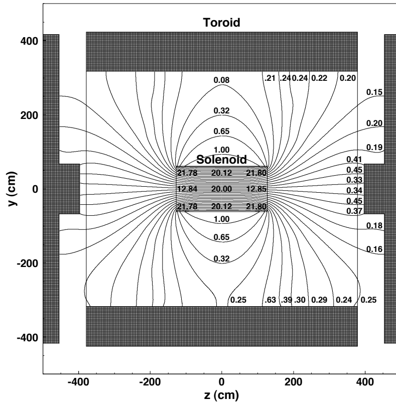
Figure 3.8: The y - z view of the D\emptyset magnetic field (in kG) with both the toroidal and solenoidal magnets at full currents (1500 A and 4749 A, respectively) [30].
