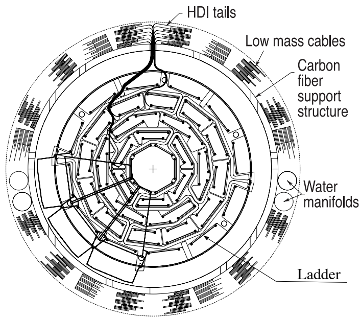
Figure 3.9: The SMT of DØ . (a) the construction of the SMT barrels and disks; (b) the ladders in a barrel.
