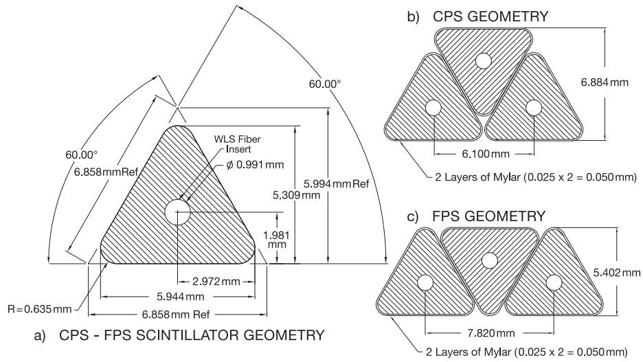
Figure 3.13: The cross section and layout geometry of the CPS and FPS scintillating fibers.
