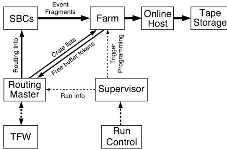
Figure 4.6: The DØ L3 DAQ and trigger system.
