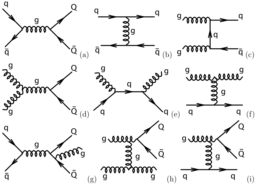
Figure 2.9: The LO and the tree level NLO representative Feynman diagrams of the b quark production in the QCD multi-jet events. (a, b) q\bar{q} LO contributions; (c, d) gg LO contributions; (e, f) gq LO contributions, notice that LO gq has no contribution if requiring two muons in the final state; (g) q\bar{q} NLO contribution; (h) gg NLO contribution; (i) gq NLO contribution.
