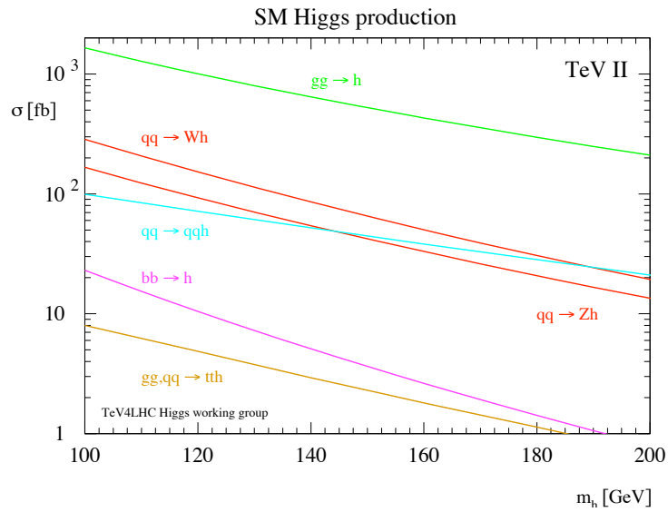
Figure 2.4: Various Standard Model Higgs boson production channel's Feynman diagrams and their cross sections at the Tevatron. The most probable channel is the gluon fusion process followed by the associated production with W and Z bosons and quark pair. The gluon fusion process and the qqh processes are experimentally uninteresting due to the large background from the QCD multi-jet process (9 orders of magnitude larger w/o the detector effects). Thus the most promising processes are the WH and ZH processes.
