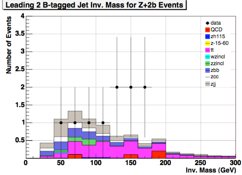
Figure 8.28: The 2 b jets' invariant mass distribution for the Z + 2 jet events double b-tag requirement. Z mass window requirement is applied.
