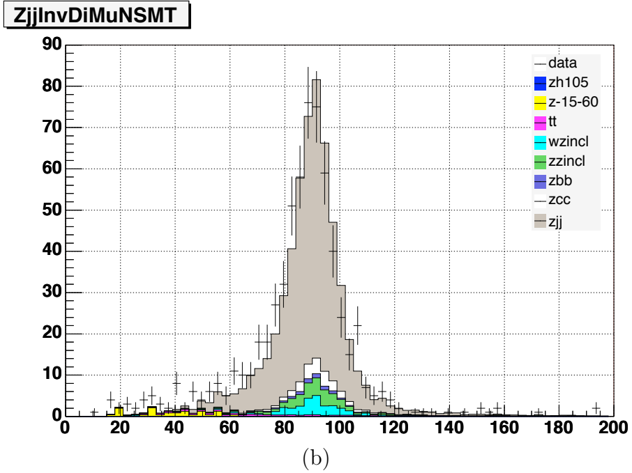
Figure 8.22: Di-muon invariant mass distribution of the Z + 2 jet with 0 btag events before (a) and after (b) the muon re-smearing. As can be seen from (a), the muon transverse momenta are over-smearing and due to the presence of the two recoil jets, the muon p_T is not well modeled, too. By re-smearing the muon momenta, these problems are solved as shown in (b).
