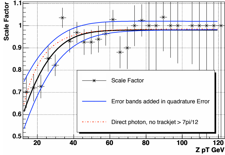
Figure 5.12: Jet RECO*ID Data/MC correction scale factor as a function of the un-smearred Z boson p_T [76].
