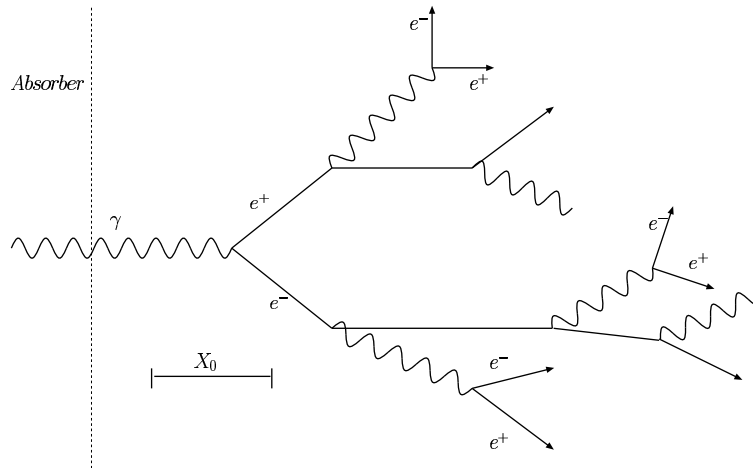
Figure 3.4: Scheme of the EM showering process. Photon pair production \gamma + \gamma^* \rightarrow e\bar{e} ( \gamma^* stands for the EM field of the material) and electron bremstrahlung e\gamma^* \rightarrow e\gamma intermingle and produce a cascading EM shower of lower energy photons and electrons.
