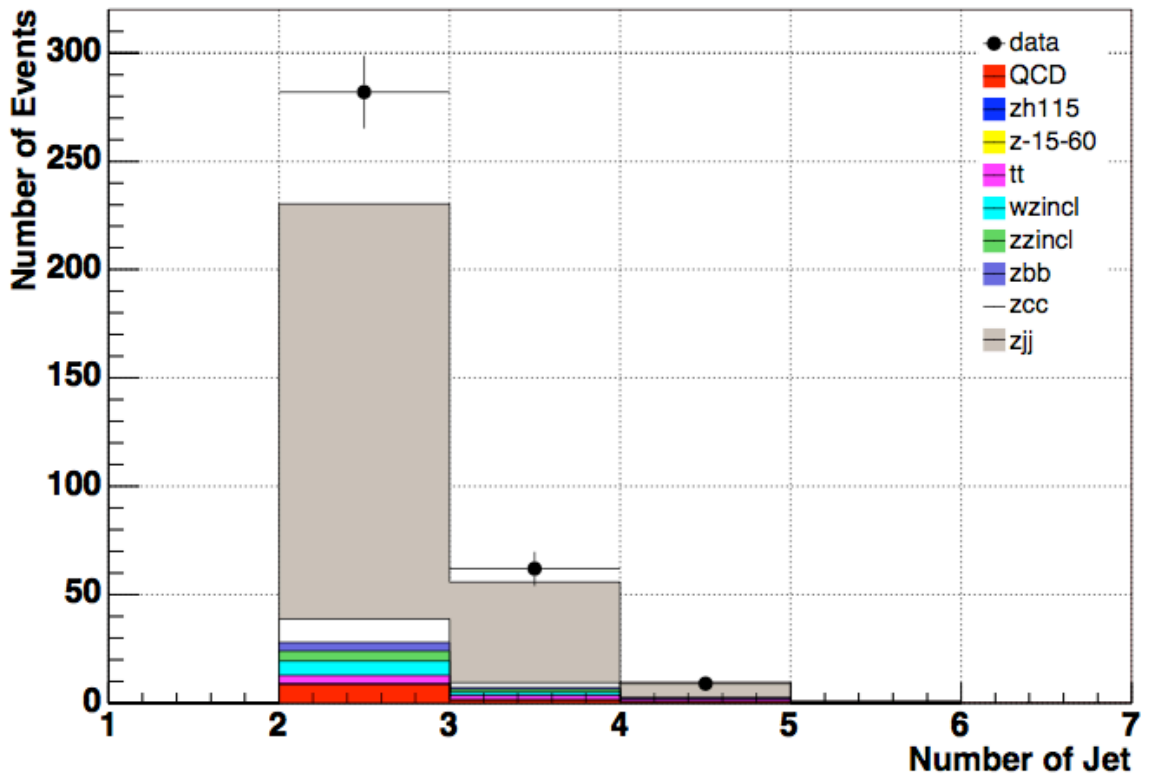
Figure 8.3: Exclusive jet multiplicity distribution for the Z + \geq 2 jet events with 0 btag.
