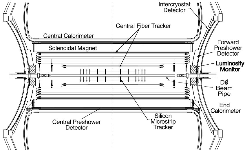
Figure 3.7: The central tracking system of D\emptyset .
