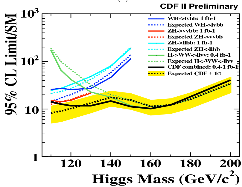
Figure 9.4: Results of the DØ and CDF Standard Model Higgs searches in different channels, (a) DØ results; (b) CDF results.
