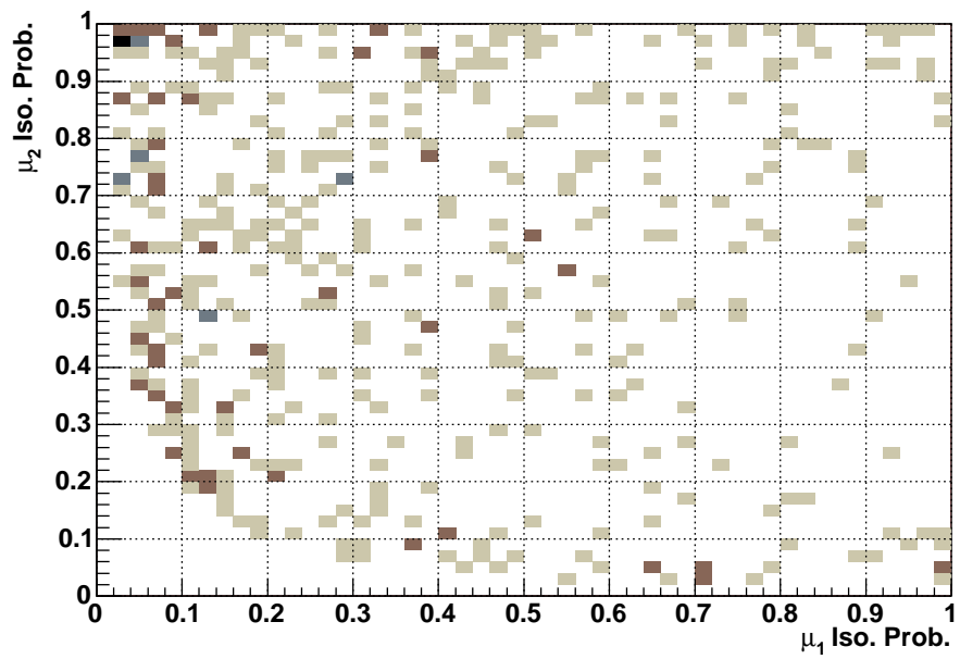
Figure 7.7: 2-D di-muon isolation probability distributions for the QCD background of 2 Z + 2 jets. The di-muon isolation probability from the QCD background are evenly distribution within the unit square. A requirement of the product of the di-muon isolation probabilities > 0.02 is applied.
