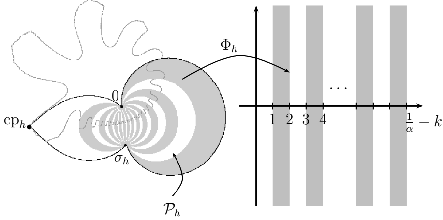
Figure 4.2: An example of a perturbed Fatou coordinate and its domain.
