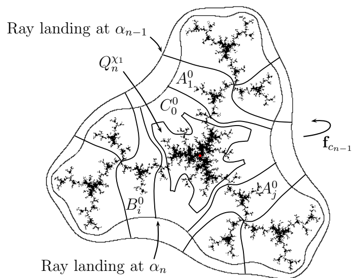
Figure 3.3: Figure of an infinitely renormalizable Julia set. The first renormalization is of satellite type and the second one is of primitive type. The puzzle piece at the center, Q_n^{X_1} , is the first puzzle piece in the favorite nest.
