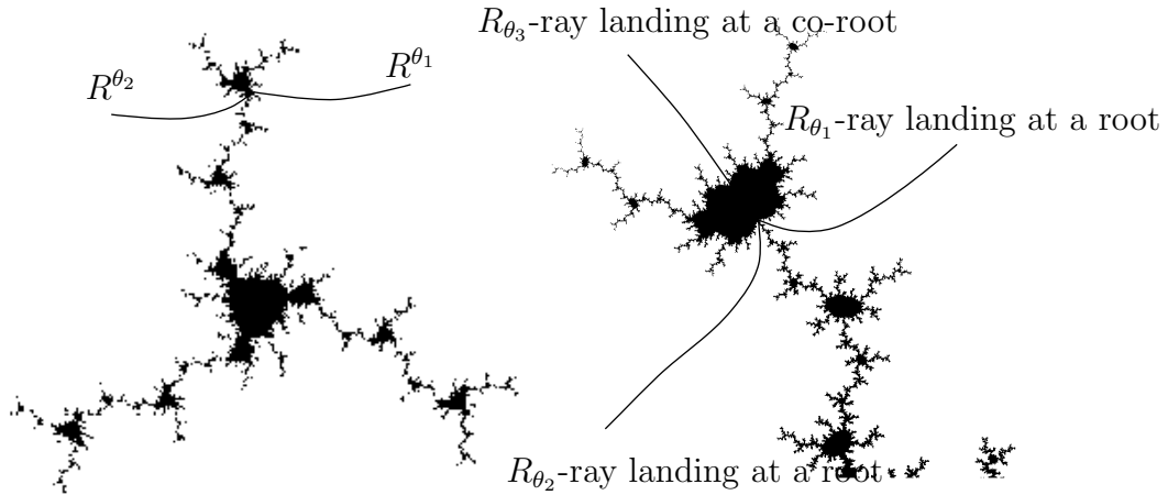
Figure 2.3: Figure on the left shows a primitive renormalizable Julia set and the external rays R^{\theta_1} and R^{\theta_2} landing at the corresponding repelling periodic point. The figure on the right is the corresponding primitive little multibrot copy. It also shows the parameter external rays R_{\theta_1} and R_{\theta_2} landing at the root point.
