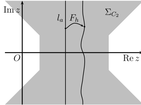
Figure 4.4: The gray region shows the domain \Sigma_{C_2} .
