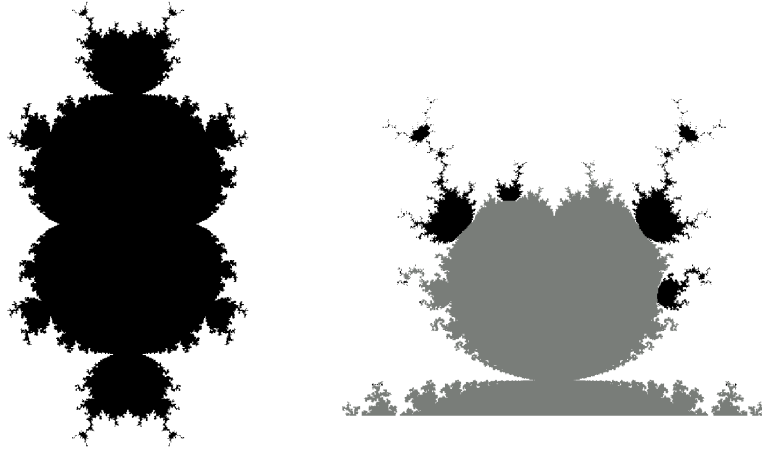
Figure 2.2: Figure on the left shows the connectedness locus \mathcal{M}_3 . The figure on the right is an enlargement of a primary limb in \mathcal{M}_3 . The dark regions show some of the secondary limbs
