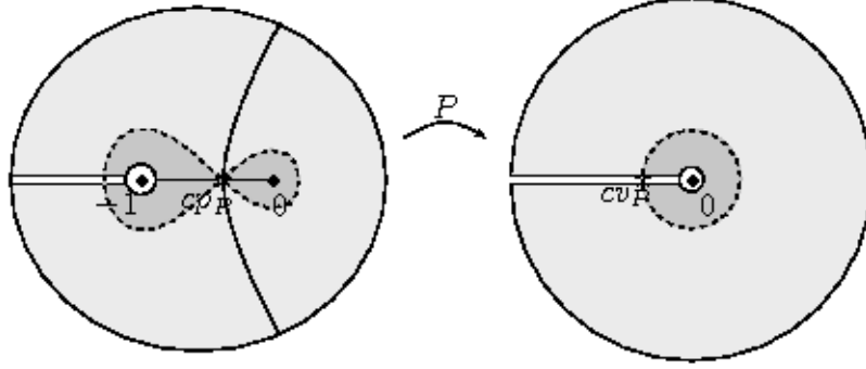
Figure 4.1: A schematic presentation of the Polynomial P , its domain, and range. Similar colors and linestyles describe the map.
