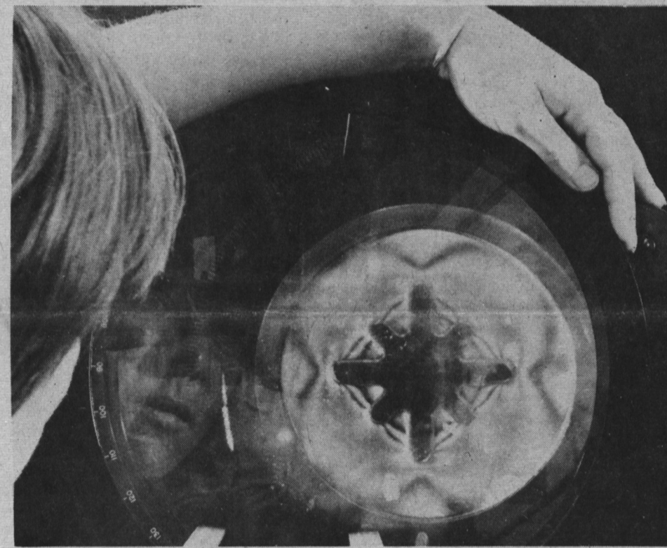
A Polariscopes study of stresses in a propeller blade model is one of 17 Open House demonstrations planned by Stony Brook's College of Engineering.
