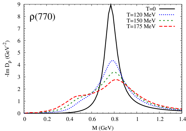
Figure 1.7: In-medium \rho spectral function as calculated with collisional broadening scenario. The \rho resonance peak “melts” as temperature increases to \simeq 175 \text{ MeV} [103] [76].
