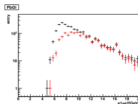
Figure 36: PbGl 2011 data
