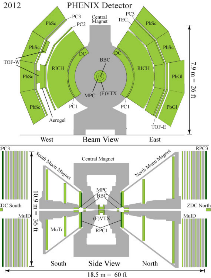
Figure 14: The PHENIX detector configuration during the 2012 data taking period. During the 2011 data taking the Forward Silicon Vertex detector was not yet installed. The top panel shows a cross section in the (x,y) plane of the central arms, while the bottom panel shows a cross section of the muon arms in the (x,z) coordinates.
