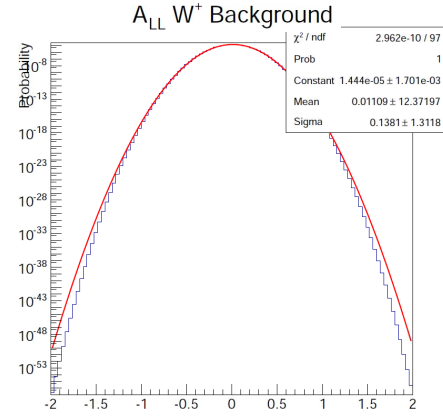
Figure 98: 2011 W^+ Background double spin asymmetry.
