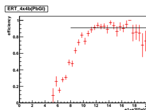
Figure 39: PbGl
