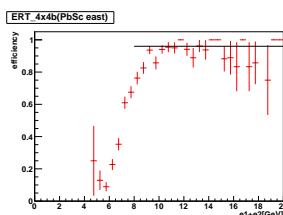
Figure 38: PbSc east
