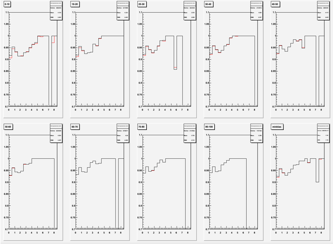
Figure 4.19: Neutron and anti-neutron correction factor ( 1 - X_{n\bar{n}} ) without any PID cut and with shower shape cut for different centralities events for PbSc.
