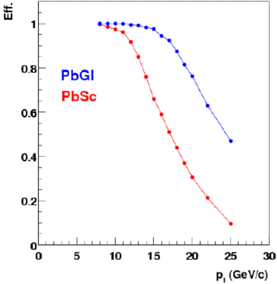
Figure 3.5: The probability that a \pi^0 is lost due to the merging inefficiency at high p_T [13].
