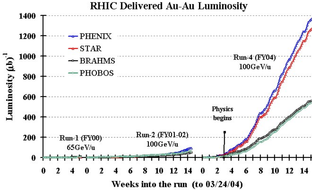
Figure 4.3: The integrated luminosity in Year-4 Au+Au run at PHENIX \sqrt{s_{NN}} = 200\text{GeV} compared to previous runs and three other detectors as a function of elapsed weeks, which indicates the data of 3.6\mu\text{b}^{-1} is recorded by PHENIX everyday on average.
