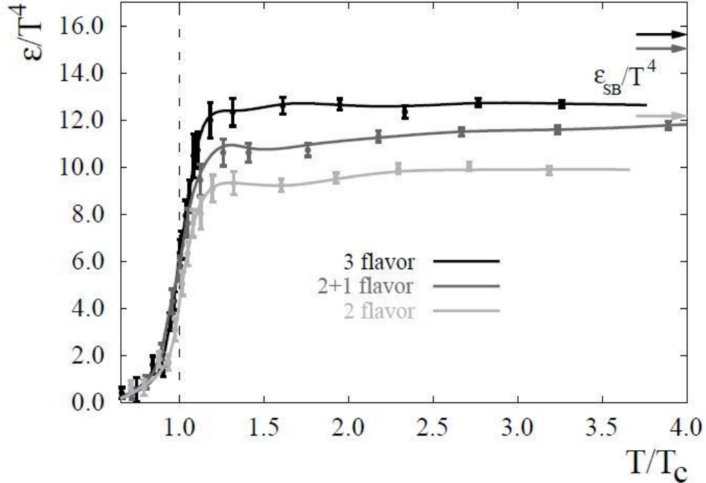
Figure 1.2: Lattice QCD results [5] for the energy density ( \epsilon ) divided by T^4 , which is degree of freedom as known from Eq. 1.2, as a function of the temperature scaled by critical temperature T_C . The arrows on the right side indicate the values for Stefan-Boltzmann limit.
