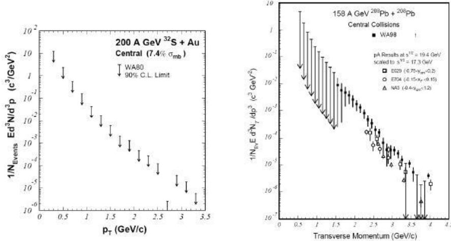
Figure 1.9: Two direct photon results in heavy ion physics before PHENIX measurement. The upper limit was set by WA80 [8] and the first measurement is by WA98 [9].
