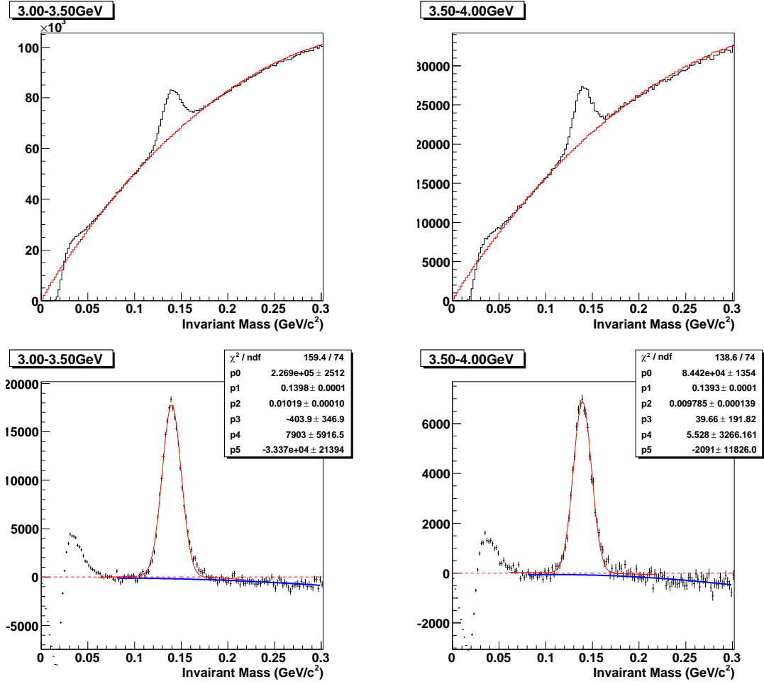
Figure C.4: Peak extraction for Stochastic Cut2 Dataset in 3.0\text{--}3.5\text{GeV}/c and 3.5\text{--}4.0\text{GeV}/c p_T bin
