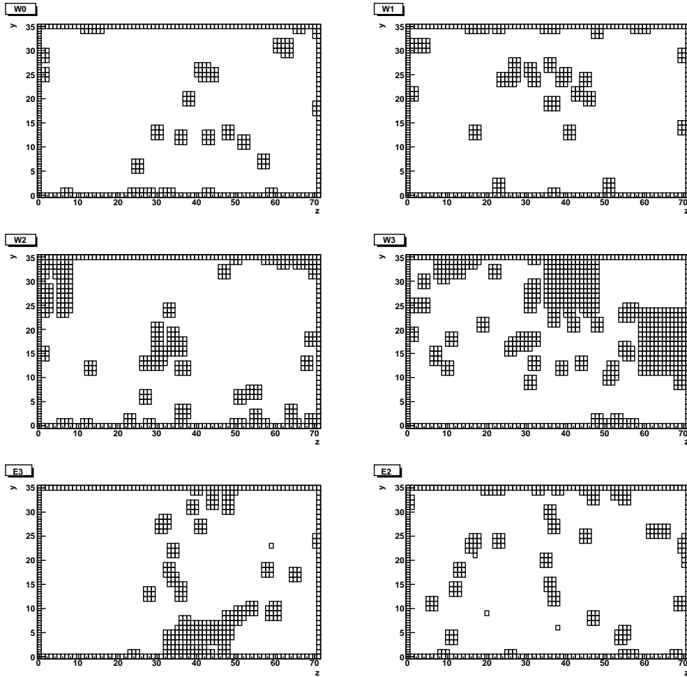
Figure B.1: Dead towers marked as boxes in the analysis for the Au+Au data. The edge towers of each sectors are also shown and excluded to reflect the fiducial cut in data analysis.
