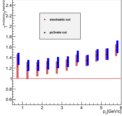
Figure 5.1: Double-ratio comparison between two different clean photon sources with different PID cuts from EMCAL for PHENIX Run4 min-bias in Au+Au \sqrt{s_{NN}} = 200\text{GeV}/c . Red is using clean photons from StochasticCut and Black is using PC3Veto plus TOF as photon PID cuts discussed in Section 4.3.2.
