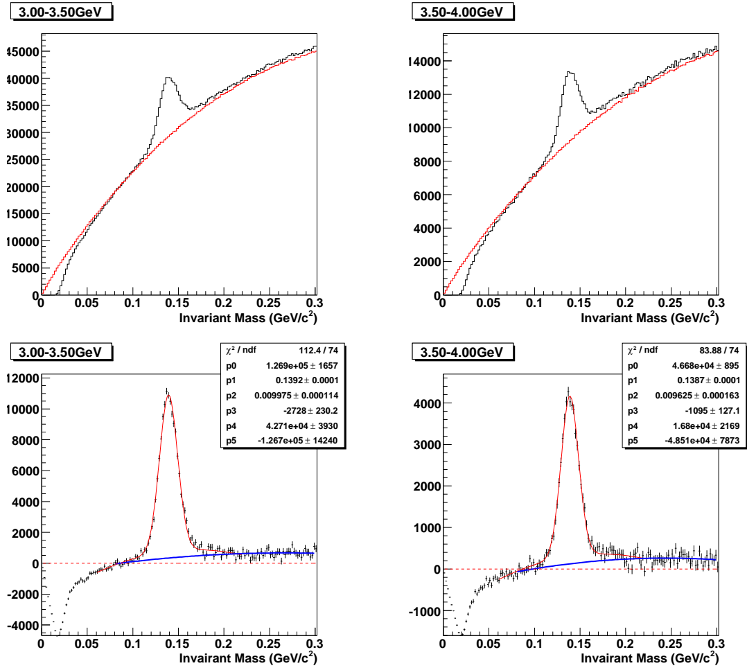
Figure D.4: Peak extraction for PC3Veto Cut Dataset in 3.0 - 3.5\text{GeV}/c and 3.5 - 4.0\text{GeV}/c p_T bin
