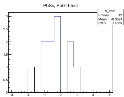
Figure A.4: Student T-scores between A_L Blue calculated in PbSc and PbGI separately.
