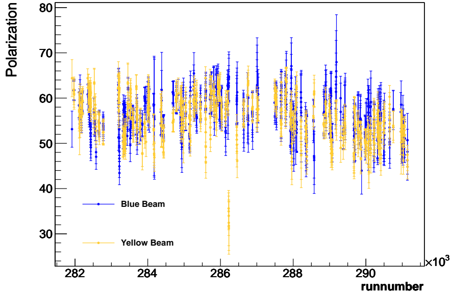
Figure 3.4: Polarization of each beam vs. runnumber, with statistical uncertainty, which was calculated from the fill-by-fill polarization values and polarization decay rates provided by the CNI-pol group. The deviation from fill-to-fill is much larger than the decay from run to run within a fill.
