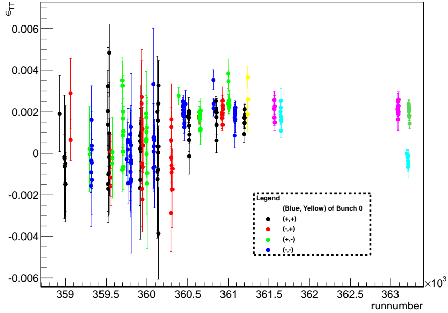
Figure 4.23: Results for the raw ZDC to BBC asymmetry in the 2012 \sqrt{s} = 200 GeV transversely polarized run with the \epsilon_N\epsilon_S\lambda method versus runnumber. The sudden change in the scatter of the points around Run 360500 corresponds to the time at which the Collider Accelerator Department turned off automatic orbit corrections.
