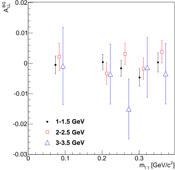
Figure 3.2: A_{LL} vs. m_{\gamma\gamma} for the background region near the \pi^0 mass peak for three p_T bins: 1 – 1.5 GeV/ c (black circle), 2 – 2.5 GeV/ c (red square) and 3 – 3.5 GeV/ c (blue triangle), for a single spin pattern in odd crossings. The peak region A_{LL} is not shown. No m_{\gamma\gamma} dependence is found.
