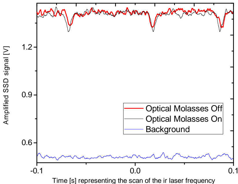
Figure 5.12: The absolute efficiency measurement data with the transverse cooling on/off. The transverse velocity spread of the atomic beam is significant to begin with, where the wider beam defining slit is used.
