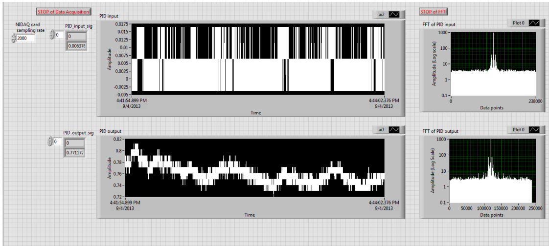
Figure 2.11: 1083 nm diode laser SAS locking signal.
