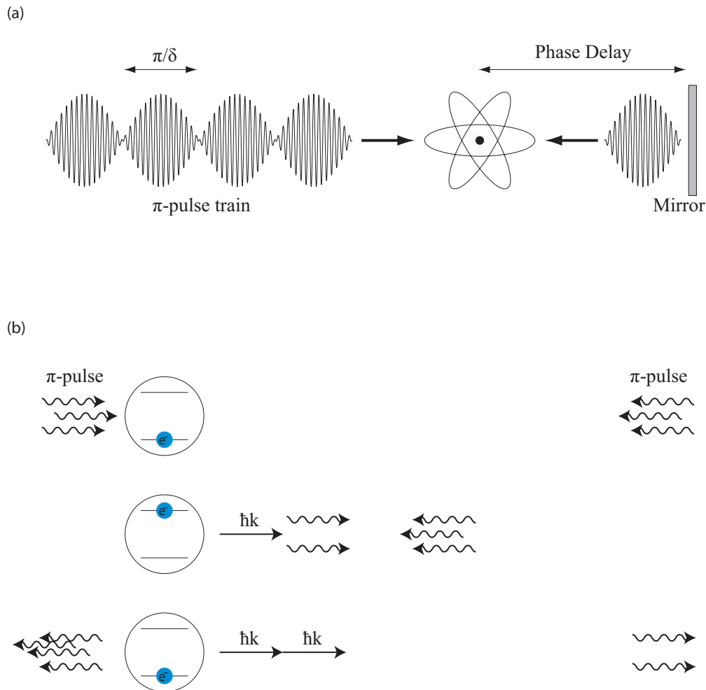
Figure 1.4: The bichromatic force explained by the \pi -pulse model. The lasers interacting with the atom can be viewed as \pi -pulse wave packets, coming from both the left and the right. The momentum exchange, and hence the force is from the stimulated emission caused by the second \pi -pulse. See also [27].
