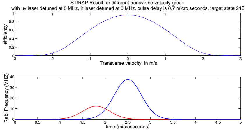
Figure 5.5: The numerical simulation of the STIRAP efficiency (as how much population ends up in the final state) for different transverse velocity groups. The ir and uv laser pulses are in STIRAP configuration, whose Rabi frequencies are shown in red and blue respectively (ir is ahead of uv). We use the Hamiltonian as in Fig. 5.4 and no polarization effect is considered. The effect of spontaneous emission is not included either.
