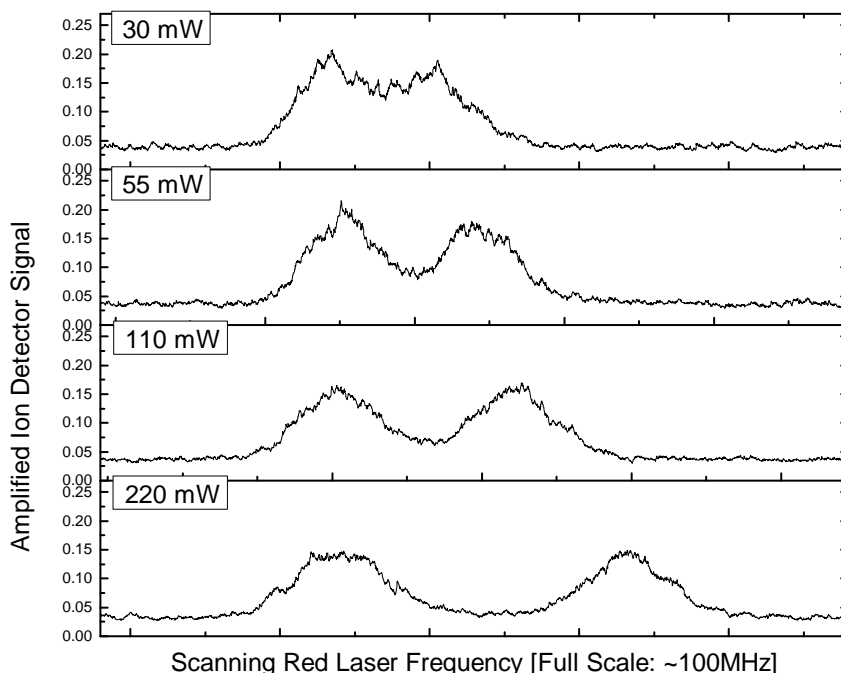
Figure 7.4: The experimentally measured Autler–Townes effect, showing the splitting caused by the uv laser Rabi frequency.
