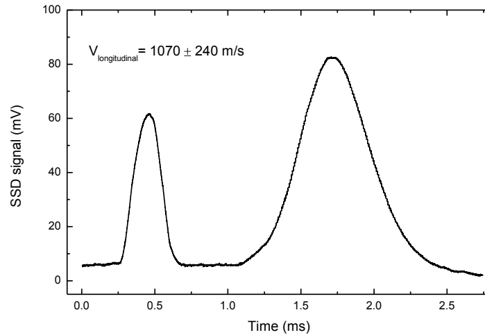
Figure 5.7: Time of flight measurement for the longitudinal velocity distribution. The source outputs both uv stray light and He*. A chopper selects a portion in the beam line and lets it travel downstream. The SSD in the detection chamber collects the signal as a function of time. The first narrow peak is the SSD’s response to the uv light and shows the time resolution of the system. The second wide peak demonstrates the longitudinal velocity distribution.
