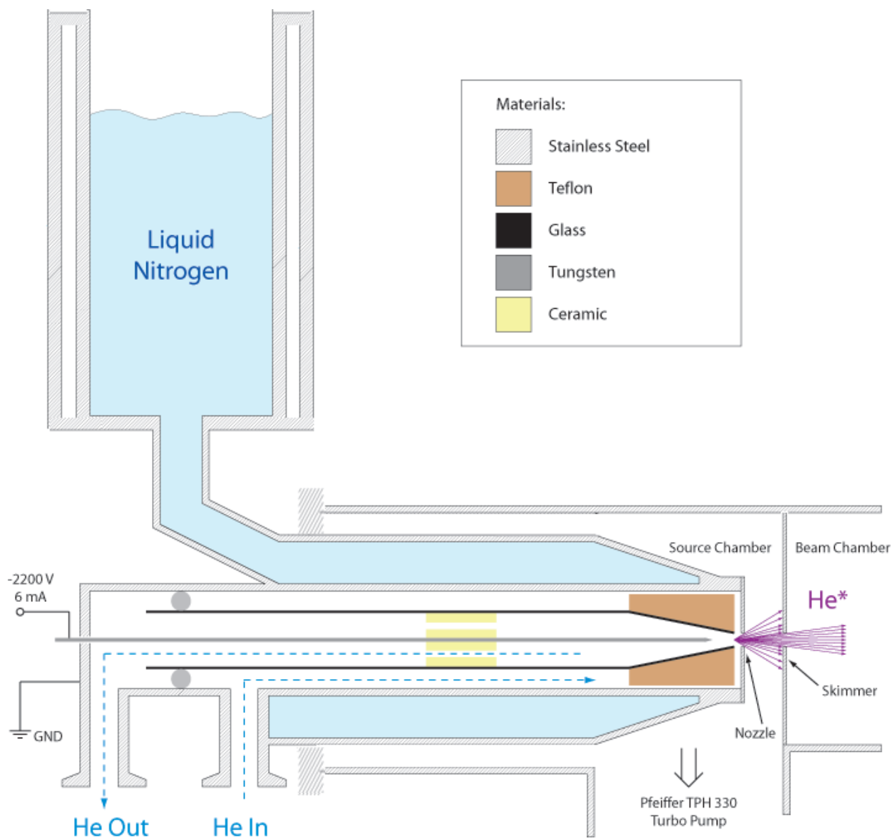
Figure 2.2: Schematics of the metastable helium source chamber. This helium gas is designed to go through a backflow. The helium is guided to be in good thermal contact with the wall of the jacket which is cryogenically cooled by the liquid nitrogen. The metastable helium is generated from an electric discharge process, with -2200\text{ V} supplied to the tungsten needle while the nozzle plate is grounded.
