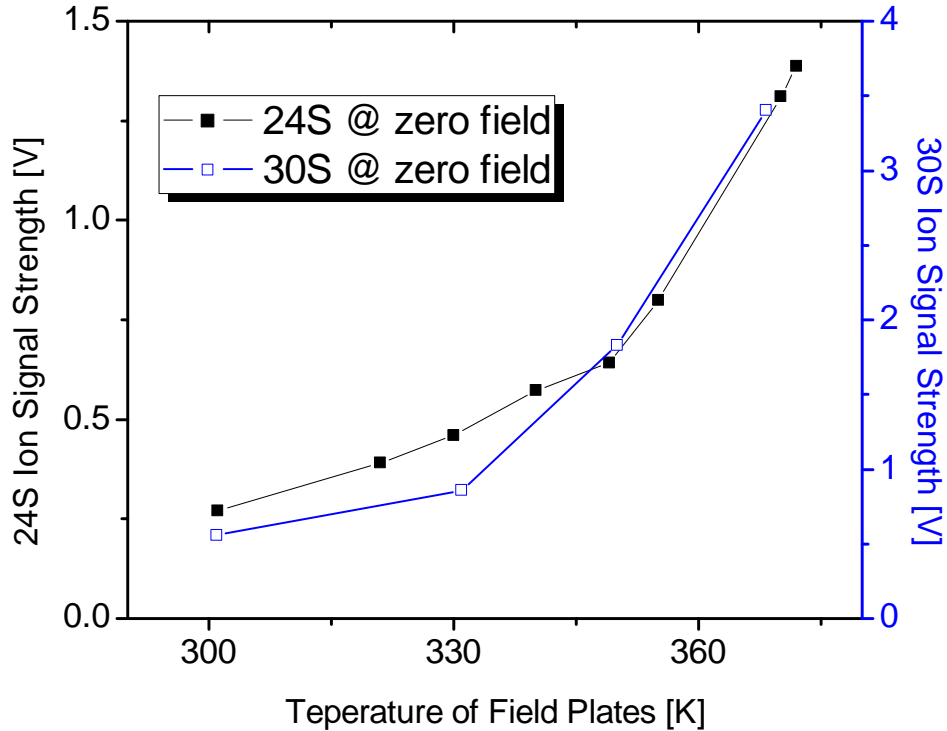
Figure 4.8: The relation of the ion signal strength and the temperature for 24^3S and 30^3S . Both measurements are at zero electric field, hence there is no concern about the electric field messing up the states or participating in the ionization process. The error bar of the ion signal is smaller than the size of the scatter and therefore is not shown.
