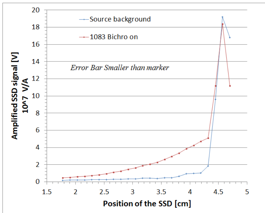
Figure 5.2: The atom profile measured by the SSD, which is scanned transversely in the detection chamber. With the 1083 nm bichromatic laser on, the atoms receive the bichromatic force and get deflected, resulting in a physical separation between the pushed metastable atoms and the center. What’s left in the center is mostly the stray uv light from the source discharge. The wide spread of the final velocities of the atoms is an inherent signature of the bichromatic force, however, by optimizing the parameters of the bichromatic laser, even better separation between the deflected atoms and the center can be achieved.
