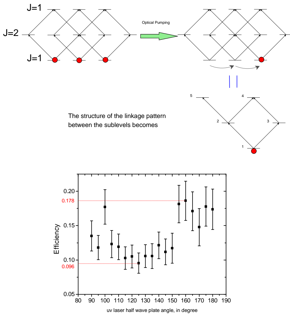
Figure 6.15: Top: the linkage pattern of the magnetic sublevels when the atom is subject to optical pumping of the 1083 nm laser first. Bottom: the measured efficiency vs. uv laser half wave plate angle.
