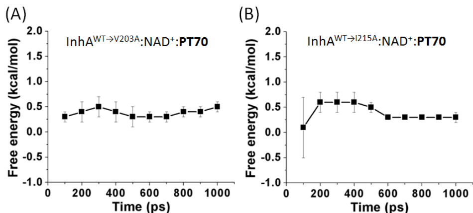
Figure 4.14. Convergence of thermodynamics integration calculation. (A) InhA WT→V203A :NAD + :PT70 (B) InhA WT→I215A :NAD + :PT70. Error bar is the difference between two independent runs. There is no significant change in the free energy after 600 ps.
