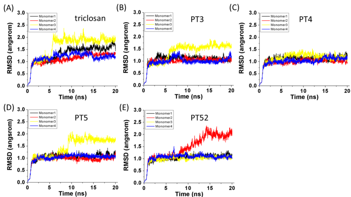
Figure 3.2. InhA backbone RMSD bound with different rapid reversible inhibitors. (A) triclosan. (B) PT3. (C) PT4. (D) PT5. (E) PT52. These simulations were started from the closed conformation. RMSD was referenced to the initial closed conformation.
