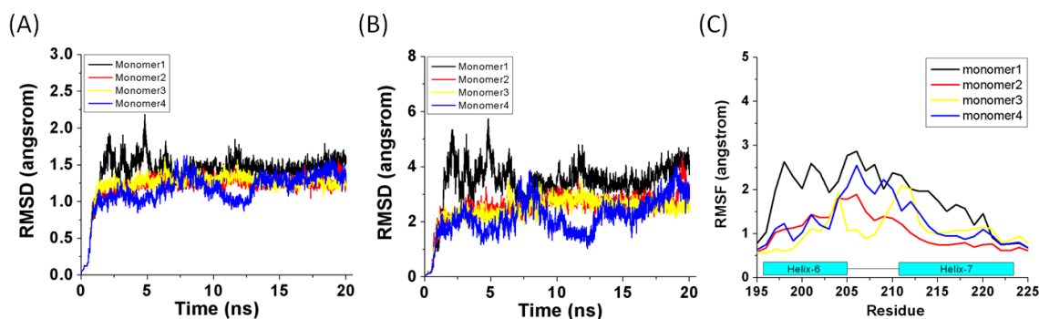
Figure 2.13. RMSD and RMSF of the InhA:NAD + :triclosan complex. (A) Backbone RMSD of the whole protein. (B) Backbone RMSD of the helix-6&7 region. (C) Backbone RMSF of the helix-6&7 region. RMSD was referenced to the open crystal structure. RMSF was referenced to the average structure.
