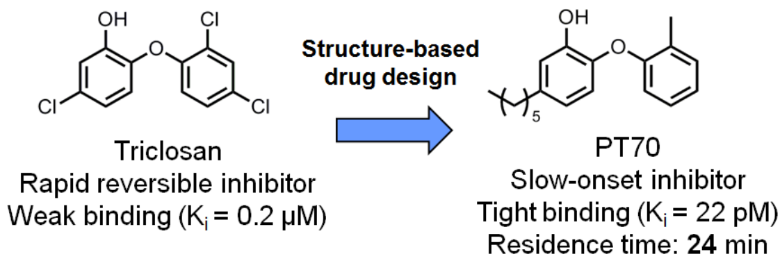
Figure 1.7. Structures of Triclosan and 2-(o-Tolyloxy)5-hexylphenol (PT70). Triclosan is a rapid reversible and weak inhibitor of InhA. Using structure-based drug design approach, PT70 was found to be a tight binding and slow-onset inhibitor of InhA.
