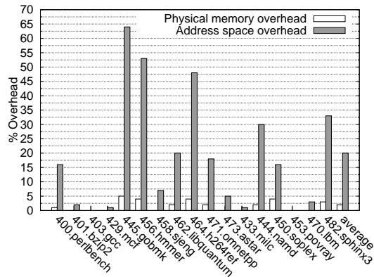
FIGURE 3.11: Space overhead of PSI on SPEC 2006
