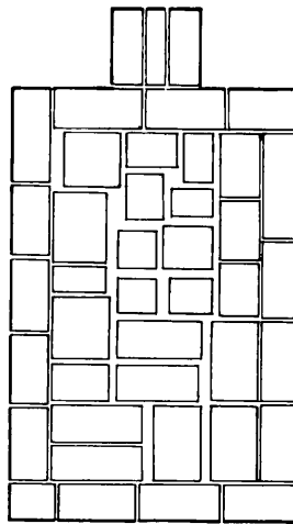
TOP FOUNDATION COURSE. LOWER COURSE SIMILAR.
